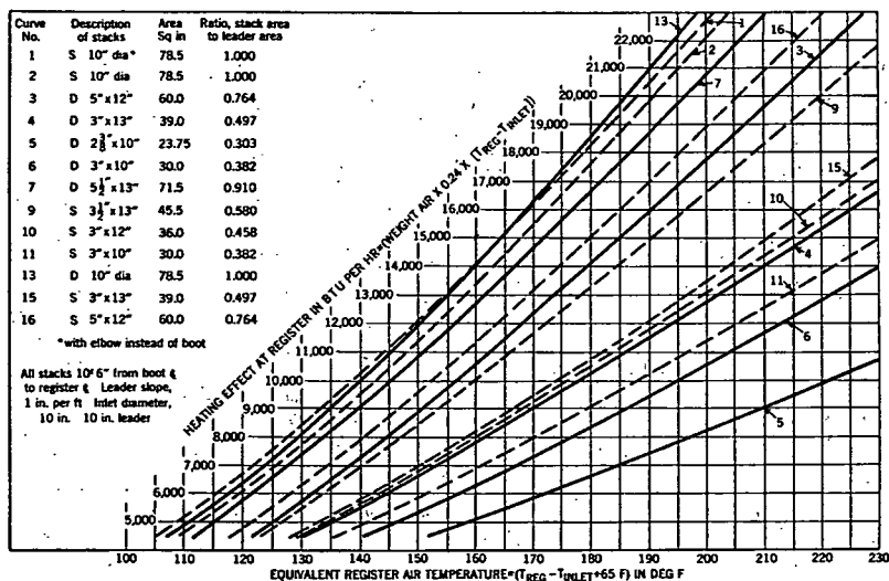
FIG. 4. HEATING EFFECT AT REGISTERS FOR VARIOUS STACKS WITH 10-IN. LEADER
