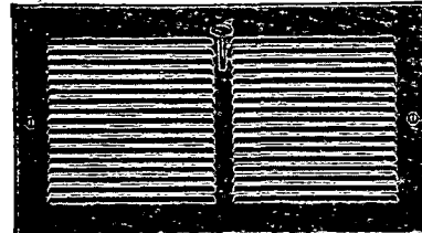
Airo-Flex No. 7032 Register—Grille bars set to direct air downward at 22 1/2 deg, but adjustable for other angles. Single louvre. Grille to match.
