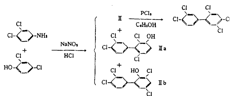
Fig. 4. Coupling Reaction of Diazotized 3,4-Dichloroaniline and 2,4-Dichlorophenol
