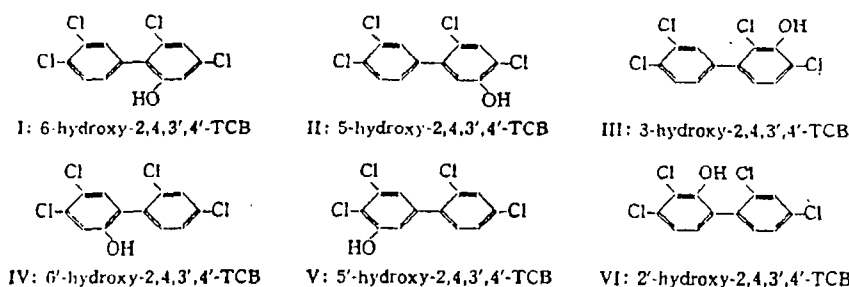
Fig. 1. Possible Isomers of Monohydroxy-2,4,3',4'-TCB
