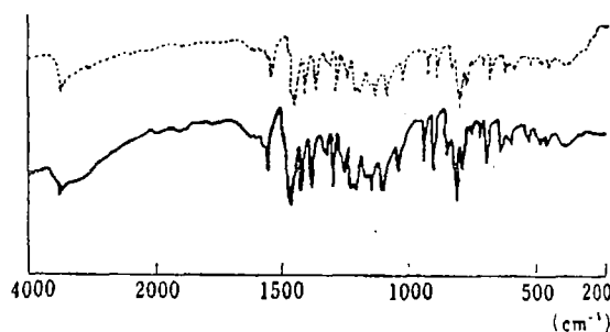
Fig. 7. IR Spectra of 3-Hydroxy-2,4,3',4'-TCB and M-A 1 1) (KBr)
