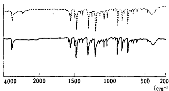
Fig. 5. IR Spectra of 5-Hydroxy-2,4,3',4'-TCB and M-A 2 1) (KBr)
