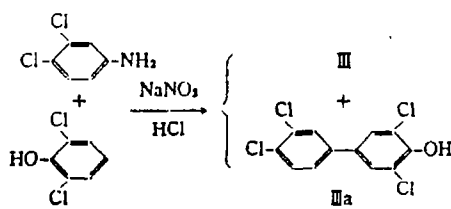
Fig. 6. Coupling Reaction of Diazotized 3,4-Dichloroaniline and 2,6-Dichlorophenol
