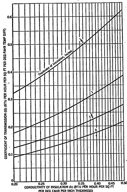
FIG. 16. HEAT LOSS COEFFICIENTS FOR INSULATED DUCTS*
