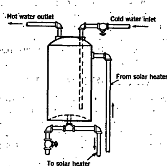
FIG. 11. SOLAR HEATER TANK CONNECTIONS
