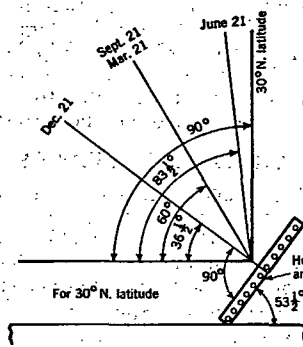
FIG. 12. SOLAR HEATING COIL INCLINATION
