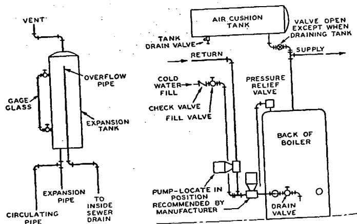
FIG. 15. AN OPEN EXPANSION TANK
