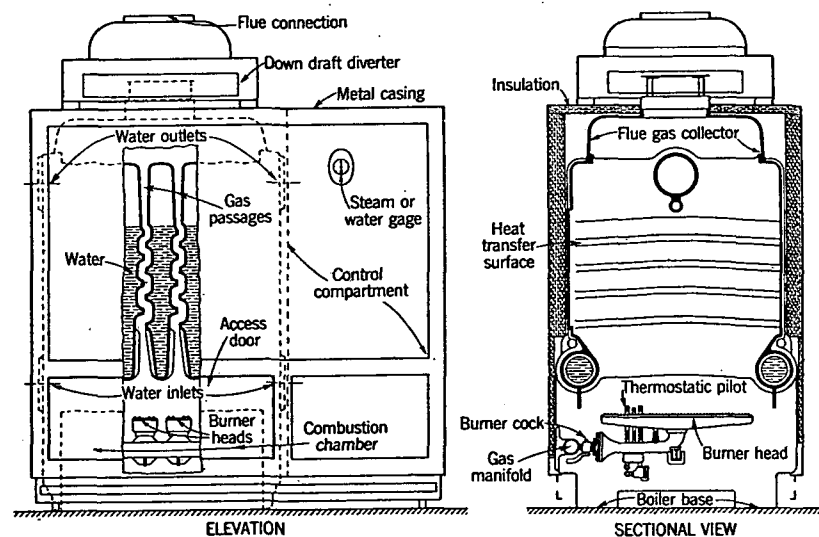
FIG. 17. COMBINATION GAS-FIRED BOILER
