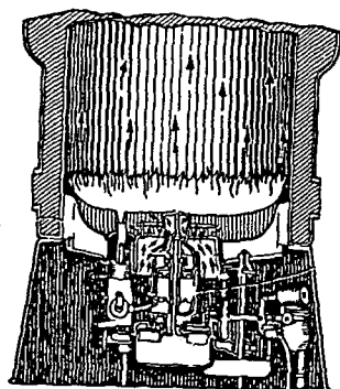
FIG. 12. CENTER FLAME VERTICAL ROTARY BURNER
