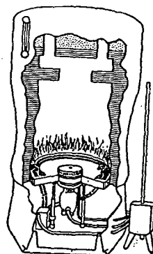
FIG. 13. WALL FLAME VERTICAL ROTARY BURNER
