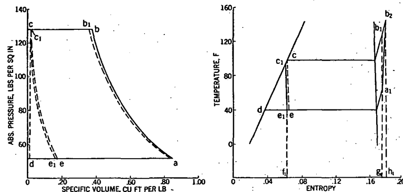
FIG. 3. PRACTICAL DICHLORODIFLUOROMETHANE (F 12 ) CYCLES
