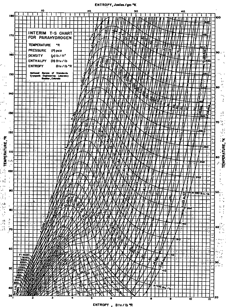
Fig. 24 .... Temperature-Entropy Diagram for Refrigerant 702 (Parahydrogen)
