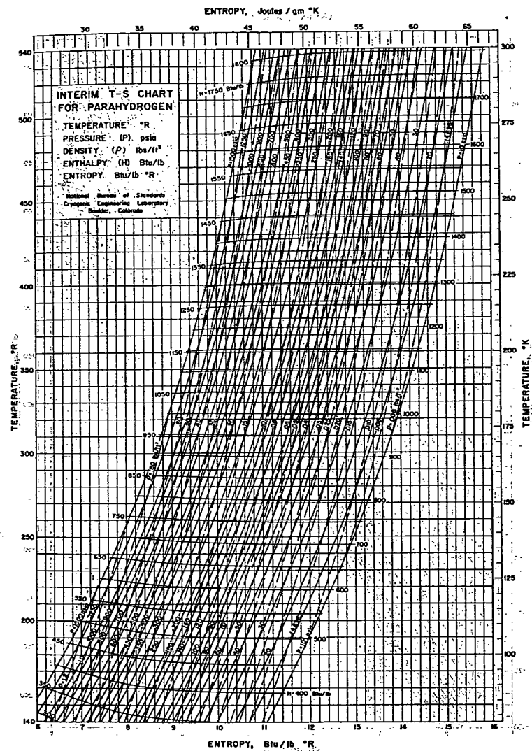
Fig. 25 .... Temperature-Entropy Diagram for Refrigerant 702 (Parahydrogen)
