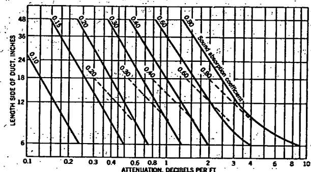
FIG. 5. SOUND ATTENUATION FOR VARIOUS ABSORBING DUCT LINERS
