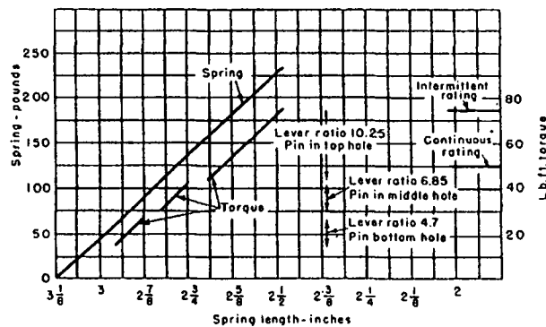
Fig. 12. Torque and spring data for IC9516-462 brake using spring Cat. No. 2415323. Normal gap = 1 inch
