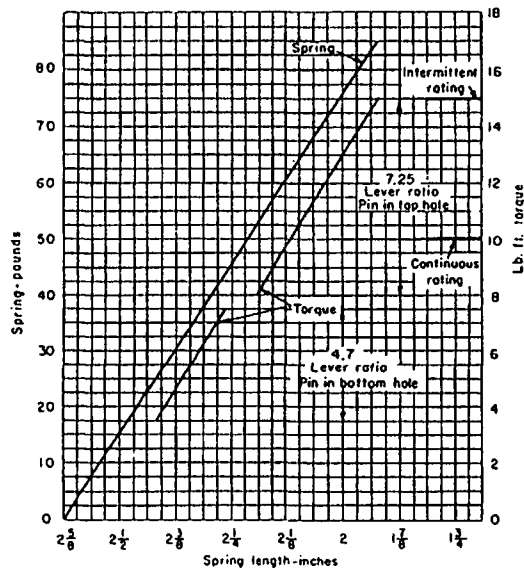
Fig. 10. Torque and spring data for IC9516-460 brake using spring Cat. No. 2415325. Normal gap = 1/2 inch
