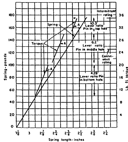
Fig. 11. Torque and spring data for IC9516-461 brake using spring Cat. No. 2415324. Normal gap = 1 inch
