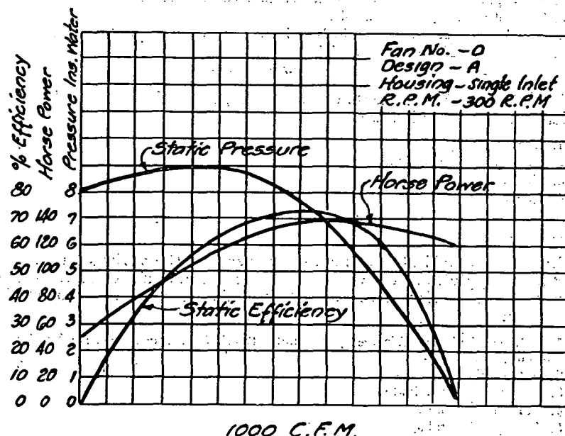
FIG. 8. TYPICAL FAN PERFORMANCE CURVE
