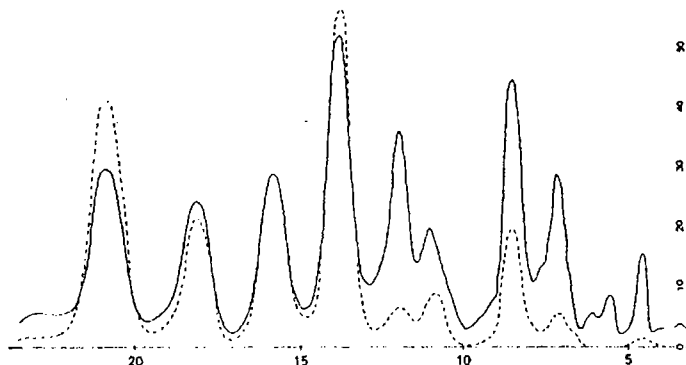
FIGURE 1. Gas chromatograms of technical Aroclor 1254 (solid line) and Aroclor 1254 residues from a Mallard egg (dotted line) of a hen maintained on feed containing 25 ppm.
