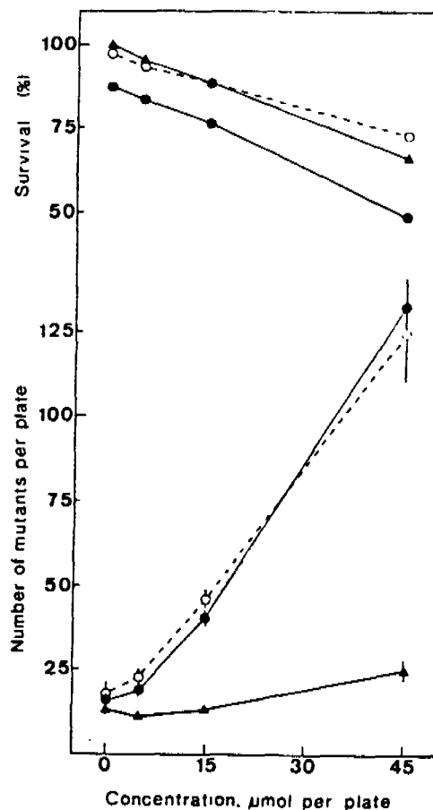
FIGURE 2. Toxic and mutagenic effects of 1,2-dichloroethane (ethylene dichloride) on Salmonella typhimurium TA 1535 (base-pair substitution) in the presence of a microsomal system with (●) or without (○) NADP or in a system with NADP but without the 9,000 \times g liver fraction (▲).
