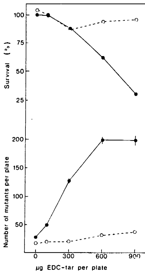
FIGURE 1 Toxic and mutagenic effects of EDC-tar on Salmonella typhimurium TA 1535 (base-pair substitution) in the presence of a microsomal system with (●) or without (○) NADP. The solvent used in this experiment was DMSO.
