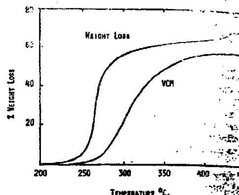
Fig. 1. PVC degradation and VCM formation as a function of temperature.
