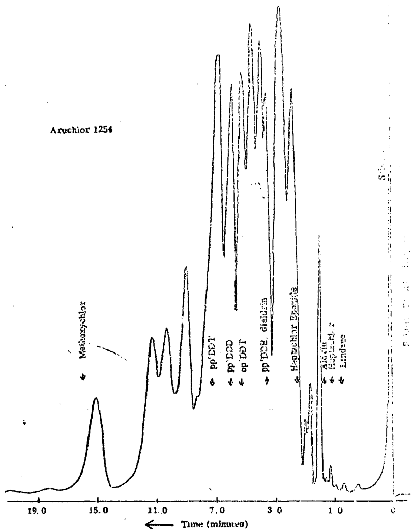
Figure 2. Commercial Mixture of Chlorinated Biphenyls
