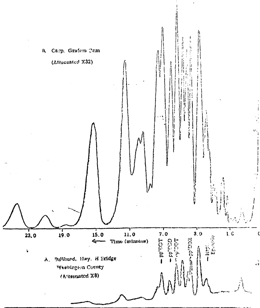
Figure 6. Fish Chromatograms from Figure 5
