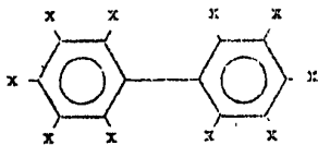
a. Chlorinated biphenyl (x indicates possible Cl positions for 1-10 Cl atoms).
