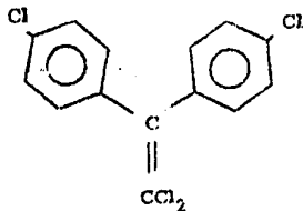
c. pp'DDE (2,2-bis(p-chlorophenyl)-1,1-dichloroethene)
