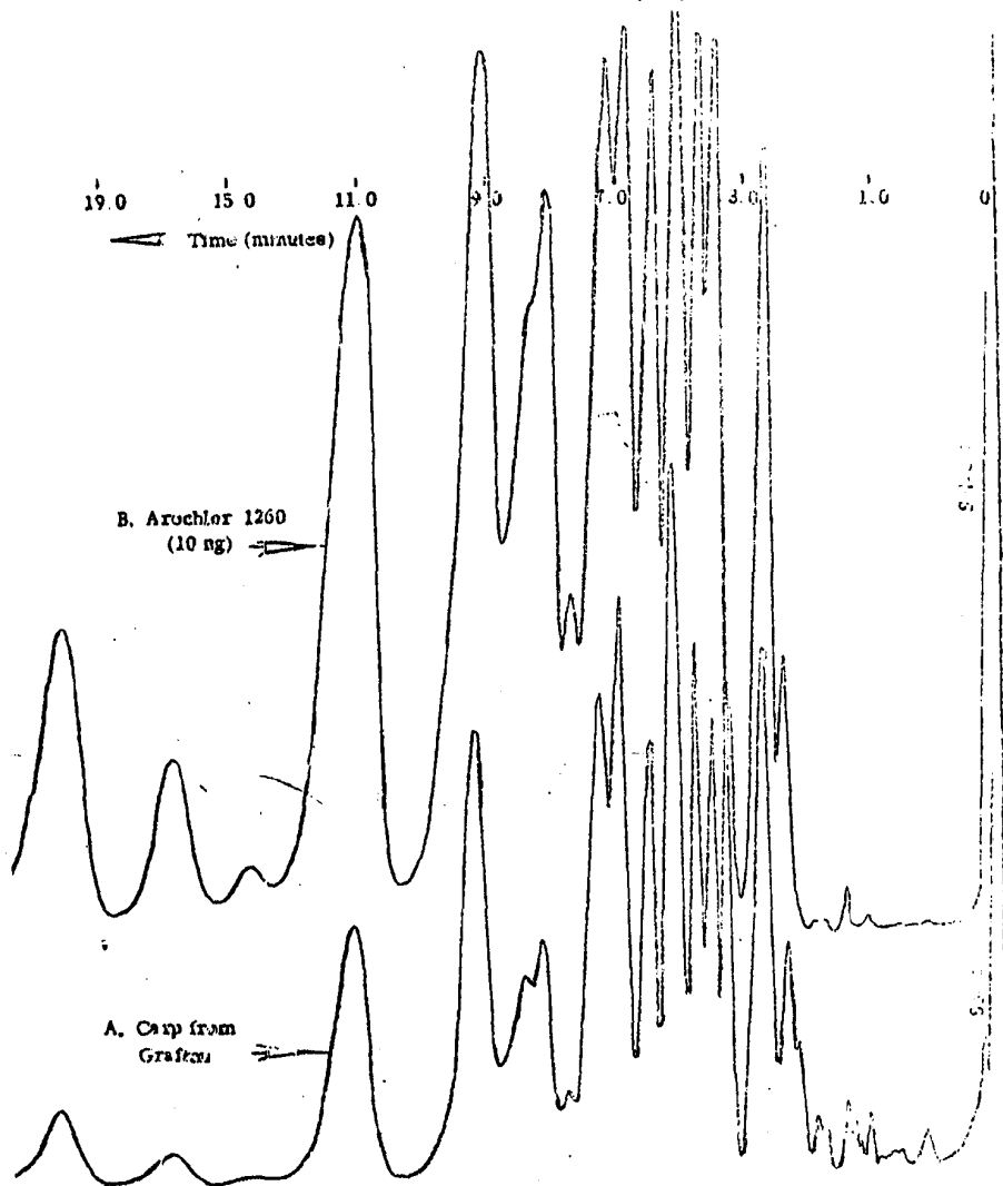
Figure 3. Comparison of the Gas Chromatograms of Aroclor 1260 Calibration Mixture
