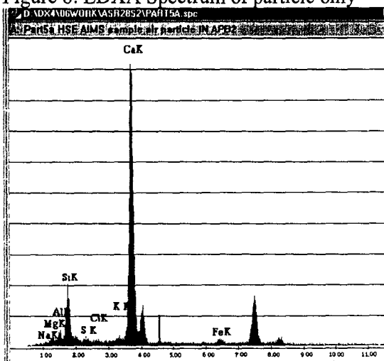
Figure 8: EDXA Spectrum of particle only
