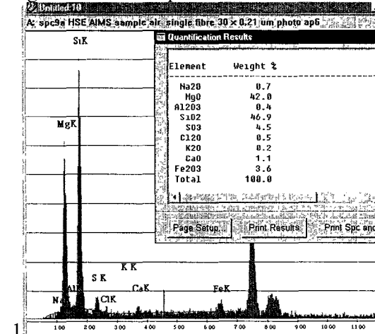
Figure 11: EDXA Spectrum from fibre
