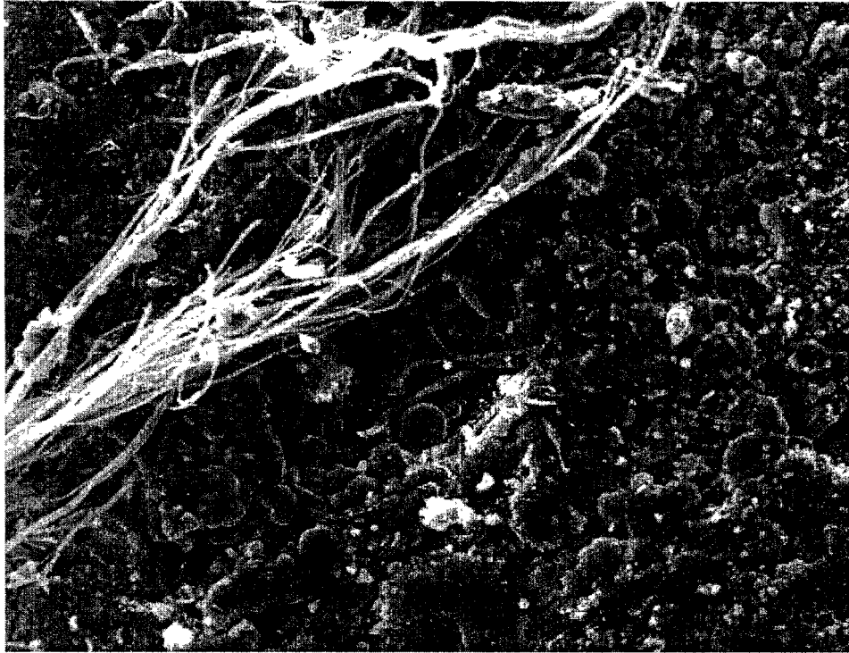
Figure 1b: Chrysotile fibre bundle exposed on the surface of a weathered cement sheet (scanning electron microscopy image at approx X600, picture courtesy of J. Dyczek). Fine cement particles are visible underneath.
