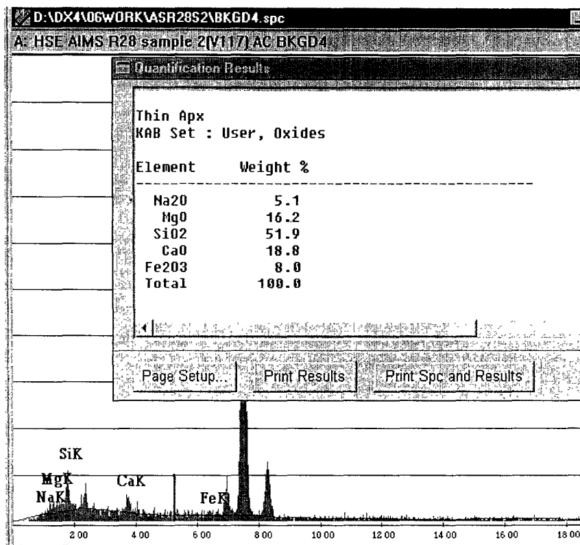
Figure 5: Example of background from the blank carbon support film near to fibre 4. (Note the weight % is relative to the height of the silicon peak which is very small compared to the EM grid peaks either side of the 8 Kev marker and only a small addition to a chrysotile spectrum will result, where the Si peak is many times greater than the EM support grid peaks).
