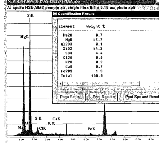
Figure 10: EDXA Spectrum from fibre
