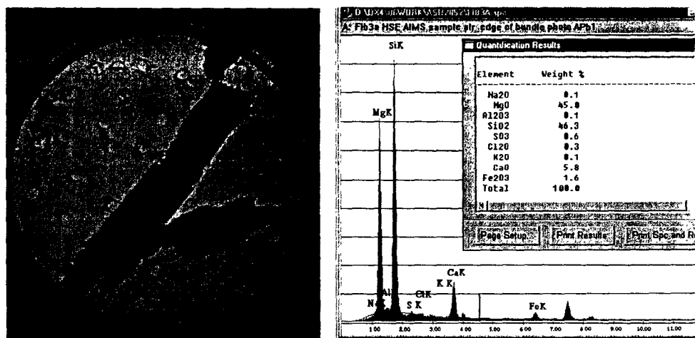
Figure 8: EDXA Spectrum of particle only
