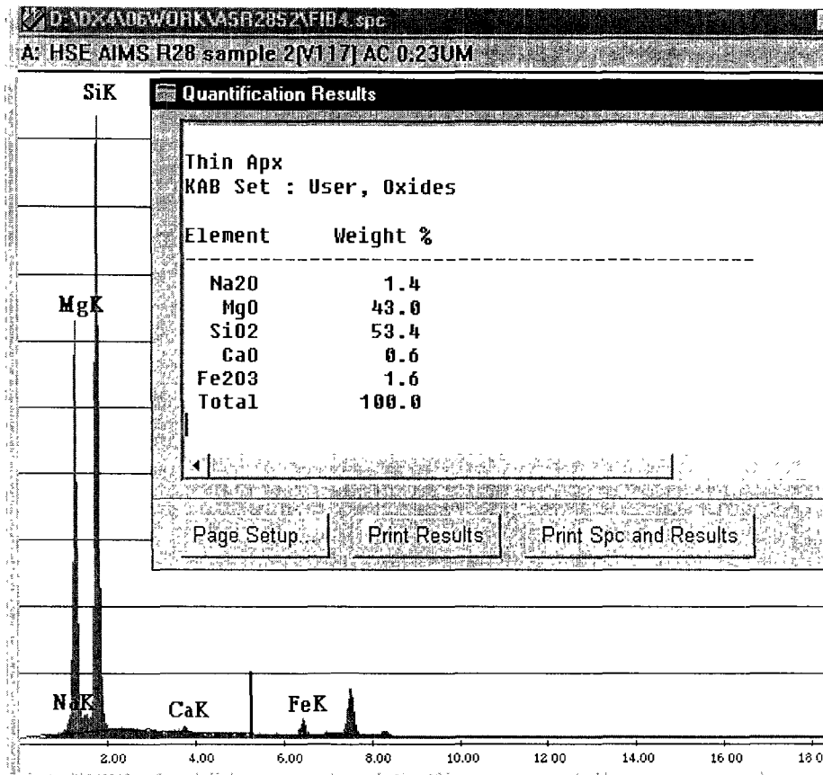
Figure 4: Energy dispersive x-ray spectrum collected from the fibre.
