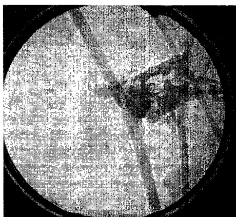
Fig 2e: Example of particle attached to chrysotile fibres. An example of the characteristic tubular structure of chrysotile can be seen. Any significant change to the chemistry is likely to be reflected by the tubular structure being broken down.
