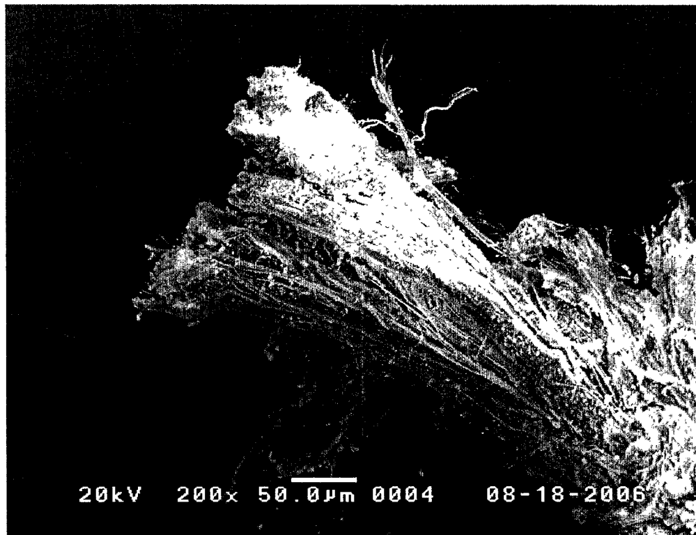
Figure 1a: Chrysotile fibre bundle projecting from a broken segment of the asbestos cement sample (scanning electron microscopy image at x200). Fine cement particles and larger pieces of matrix material can also be seen.
