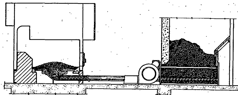
FIG. 10. UNDERFEED SCREW STOKER, BIN TYPE, CLASS 2, 3 OR 4
