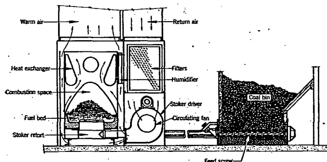
FIG. 8. STOKER-FIRED WINTER AIR CONDITIONING UNIT
