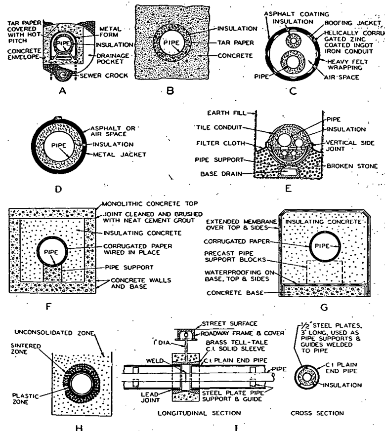
FIG. 1. A FEW TYPICAL CONDUITS FOR DISTRICT HEATING USE
