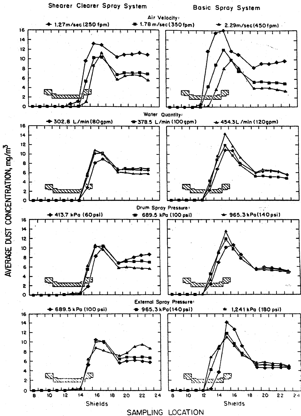
Figure 3. Dust profiles for test conditions with the shearer cutting in the tail-to-head direction.
