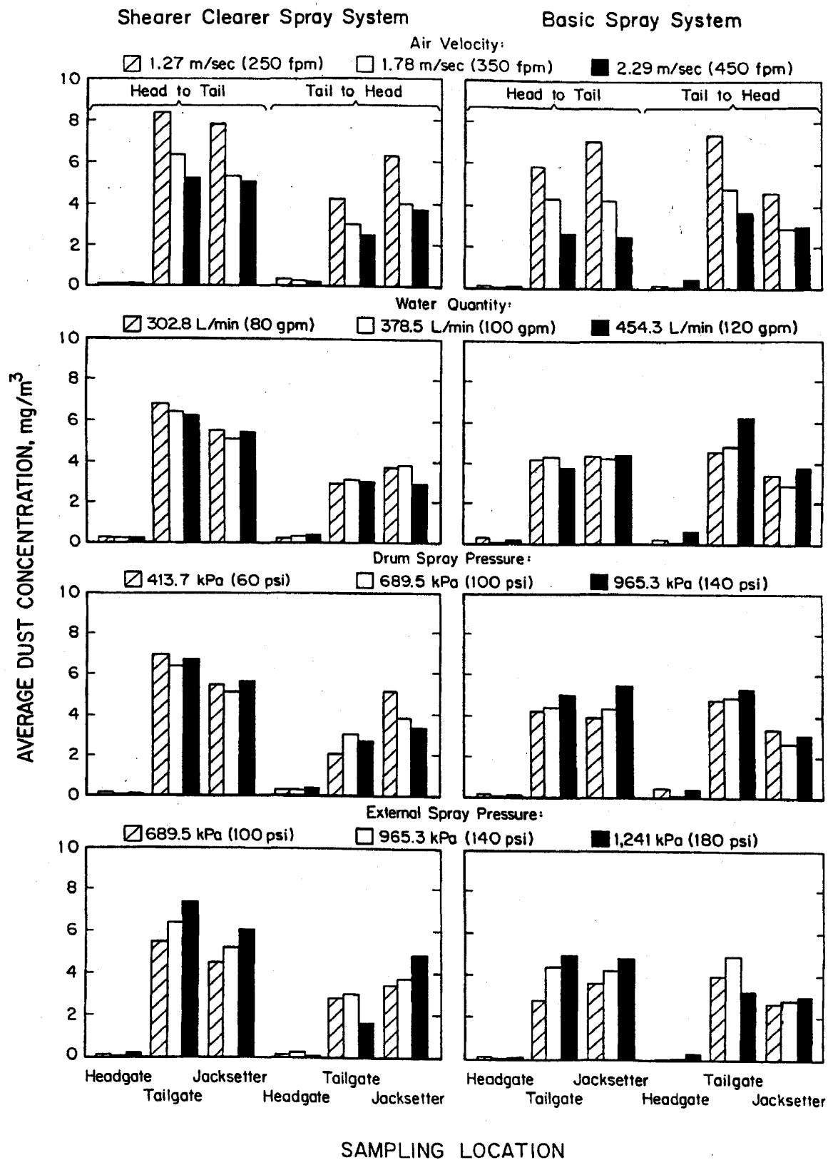
Figure 2. Summary of gravimetric sampling results.
