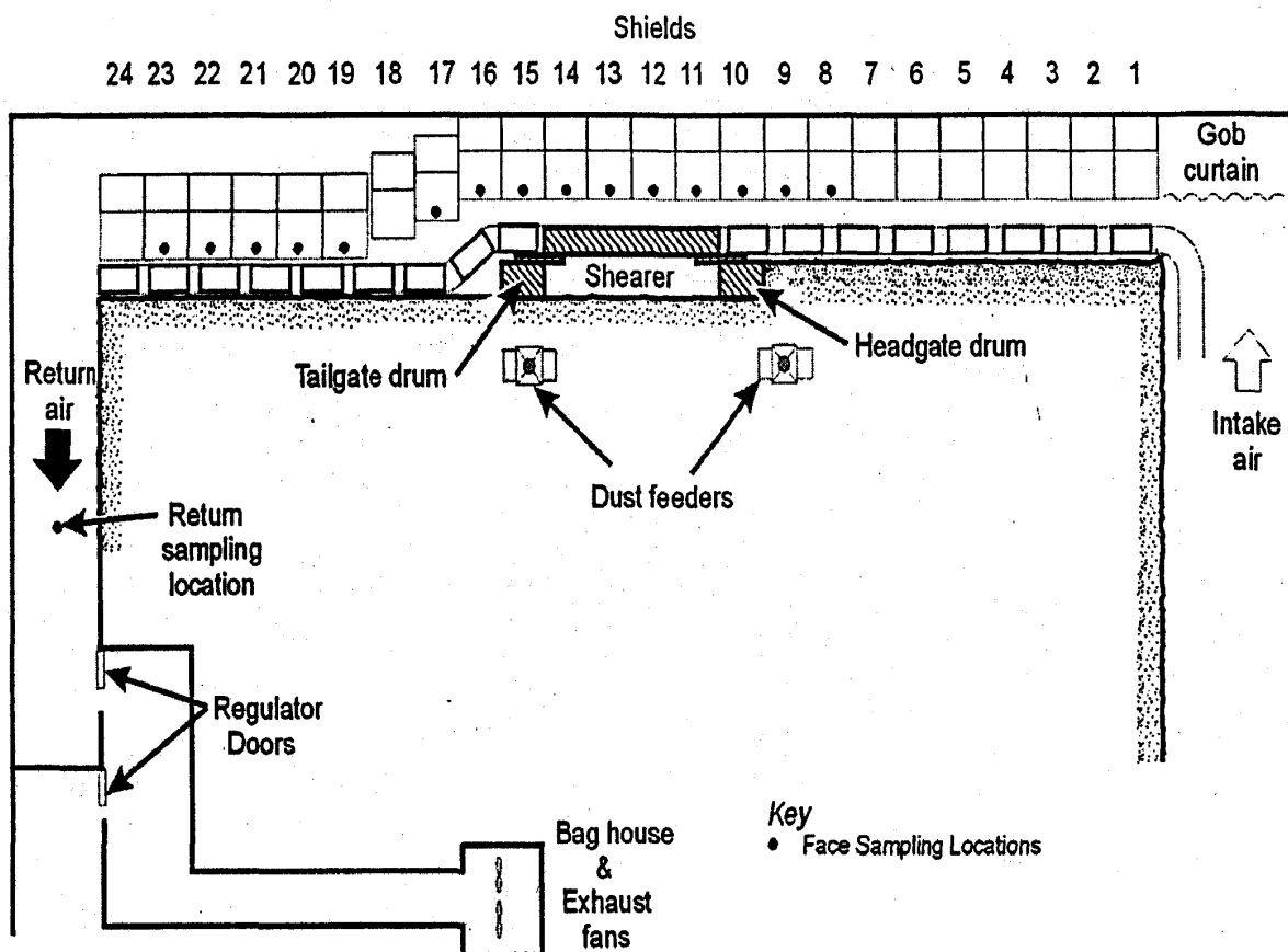
Figure 1. Diagram of longwall test facility at the Pittsburgh Research Laboratory.
