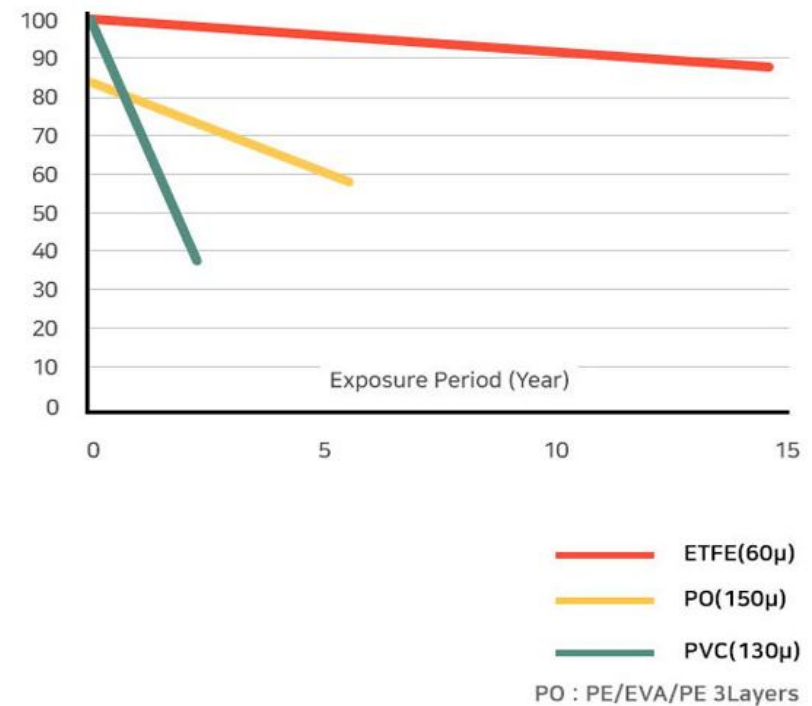
(Fig.2 Exposure period vs. Light transmission)
