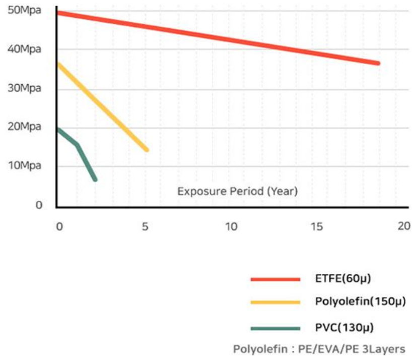
(Fig.1 Exposure period vs. Tensile strength)
