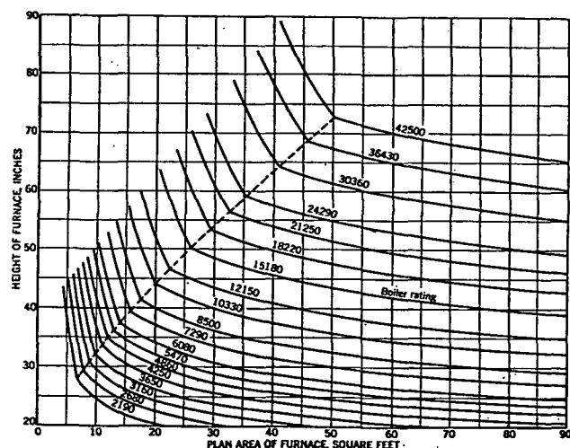
FIG. 1. FURNACE HEIGHTS FOR STOKER FIRED BOILERS AND BITUMINOUS COAL RATED IN SQUARE FEET STEAM RADIATION
