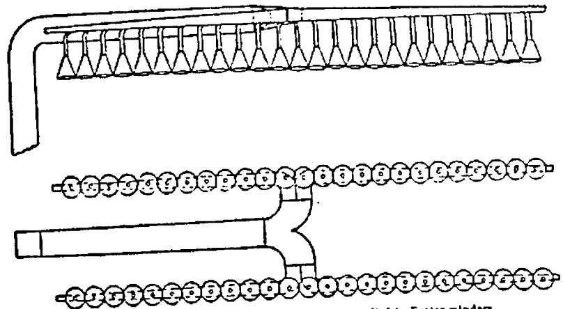
FIGURE 4.—Schematic views of exhaust system applied to Foster winders.
