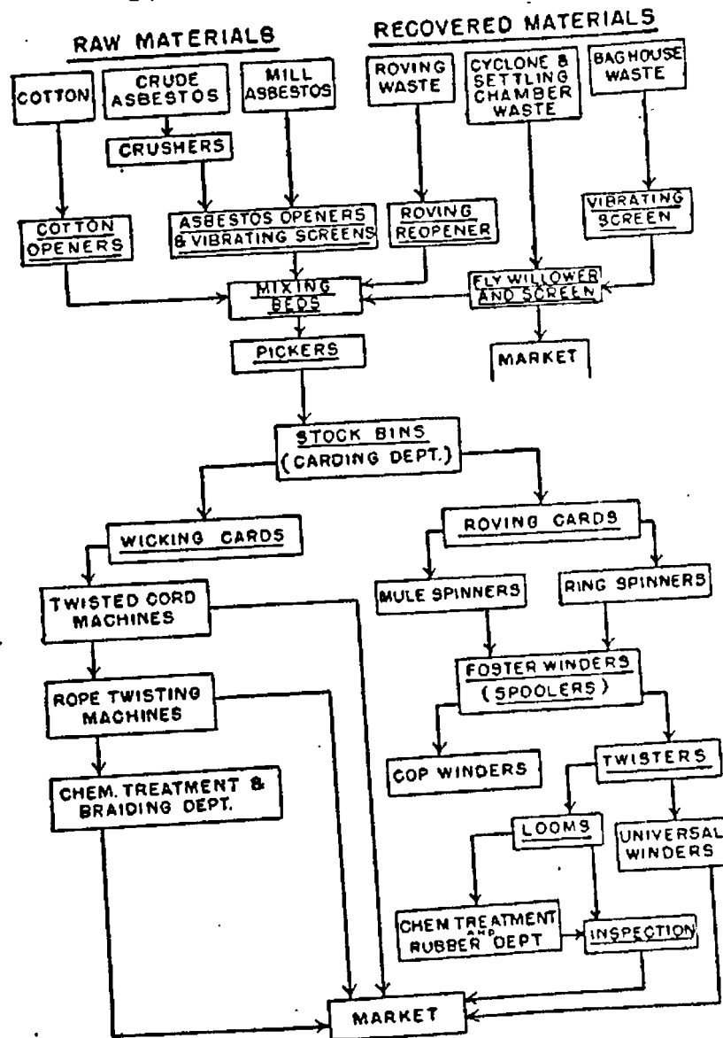
FIGURE 1.—Process flow sheet, asbestos textile plant.
