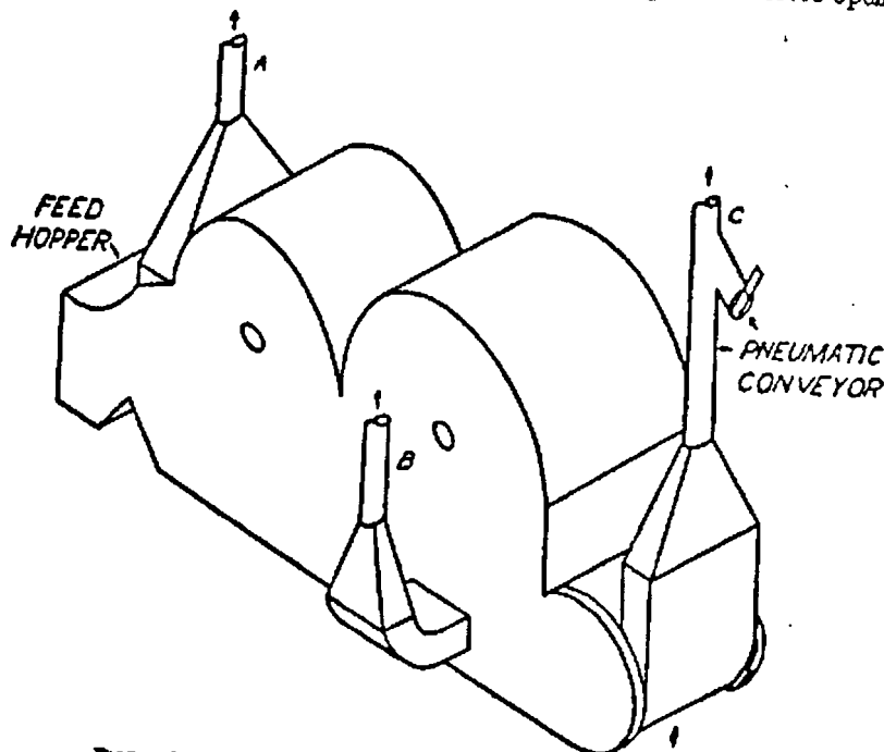
FIGURE 2.—Schematic view of exhaust system applied to an asbestos opener.
