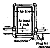
FIG. 36. LOOPING DRY RETURN MAIN AROUND OPENING
