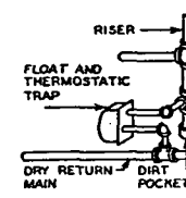
FIG. 42. DRIPPING HEEL OF RISER INTO DRY RETURN
