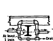
FIG. 35. LOOPING MAIN AROUND BEAM
