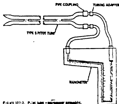
FIGURE 102-2. Pitot tube - manometer assembly.
