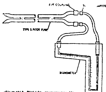
Figure 104-2. Pilot tube - manometer assembly.
