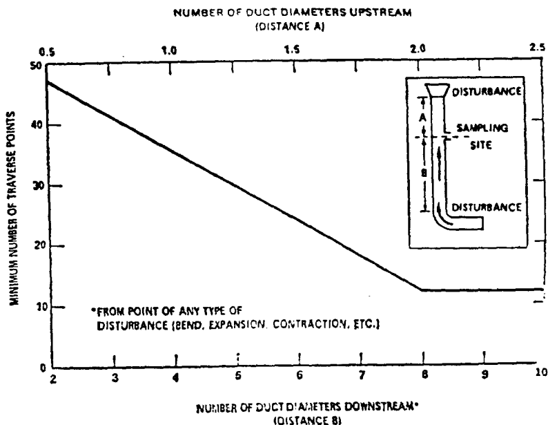
Figure 102-3. Minimum of traverse points.
