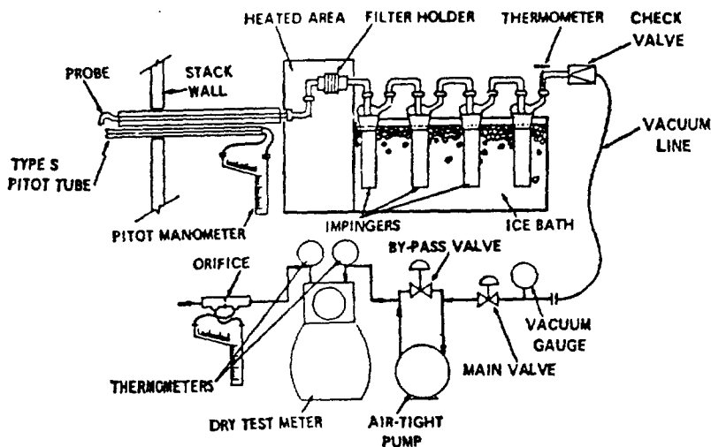
Figure 104-1. Beryllium sampling train
