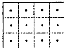
Figure 104-5. Cross section of rectangular stack divided into 12 equal areas, with traverse points at centroid of each area.
