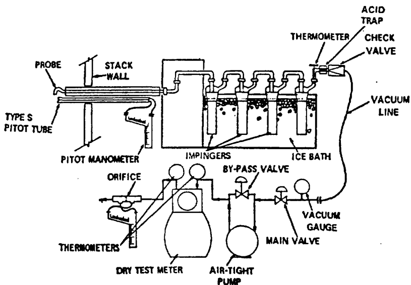
Figure 102-1. Mercury sampling train
