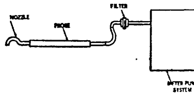
Figure 103-1. Beryllium screening method; sample train schematic.
