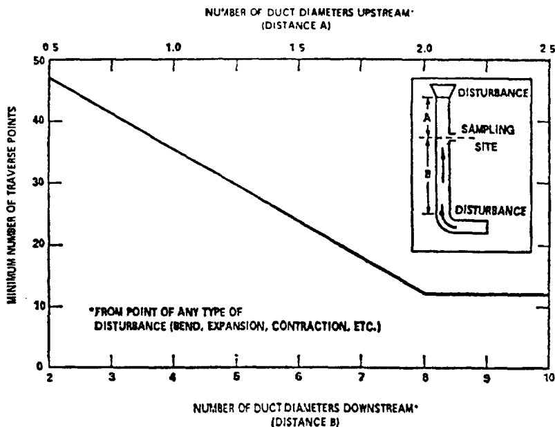
Figure 104-3. Minimum number of traverse points.
