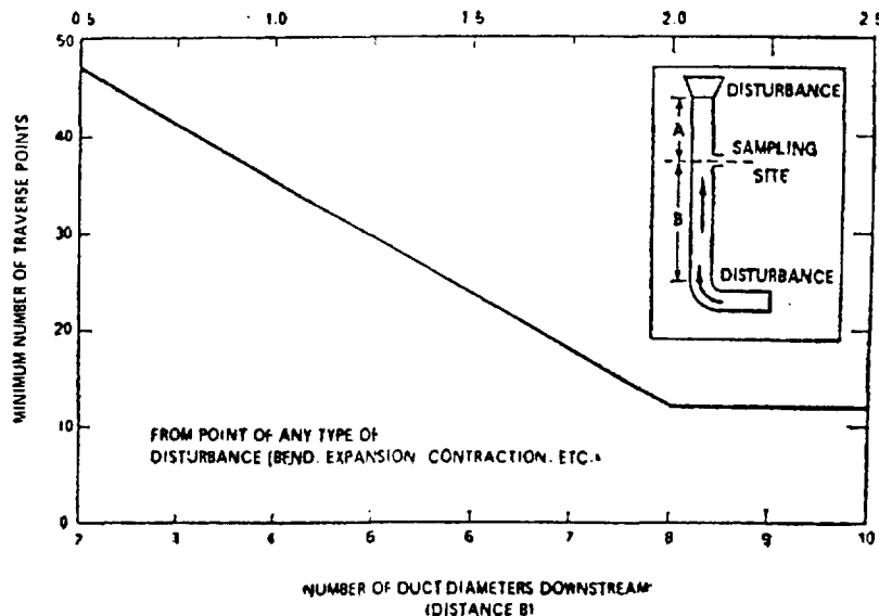
Figure 104-3. Minimum number of traverse points.
