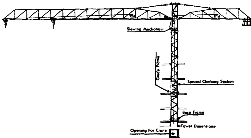
CLIMBING-TYPE CRANE
