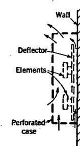
FIG. 2. CONVECTOR HEATER
