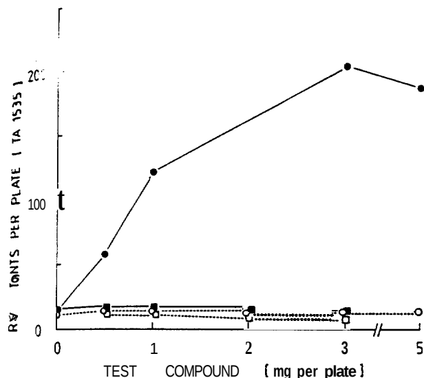
FIGURE 3. Mutagenicity of trans -benzene-1,2-dihydrodiol (●, ○) and catechol (■, □) in Salmonella typhimurium TA1535 in the presence (closed symbols) and absence (open symbols) of NADPH-fortified post-mitochondrial supernatant (S9) fraction from liver homogenate of Aroclor 1254-treated male Sprague-Dawley rats. The plate-incorporation protocol was used and each plate received S9 equivalent to 100 mg liver tissue. Details of the assays were as described previously (4).
