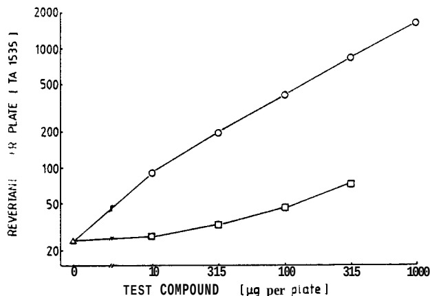
FIGURE 4. Mutagenicity of anti-benzene-diol epoxide (○) and syn -benzene-diol epoxide (□) in Salmonella typhimurium TA1535. The test compound (dissolved in 10 \mu L dimethylsulfoxide:triethylamine, 1000:1), 100 \mu L of the bacterial resuspension ( 1.04 \times 10^8 colony forming units) and 500 \mu L buffer (150 mM KCl, 10 mM sodium phosphate buffer, pH 7.4) were incubated for 20 min at 37°C. Soft agar was then added and the mixture poured onto minimal agar plates (27). After incubation for 3 days at 37°C in the dark, the colonies were counted. Values are means from two plates, the average standard deviation being 10.7% of the mean.
