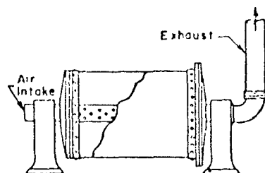
FIGURE 127. Local Exhaust Ventilation at a Hollow-Trunnion Type Tumbler
