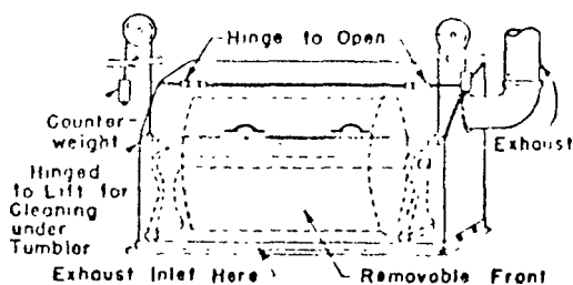
FIGURE 128. Enclosure and Local Exhaust at a Tumbler
