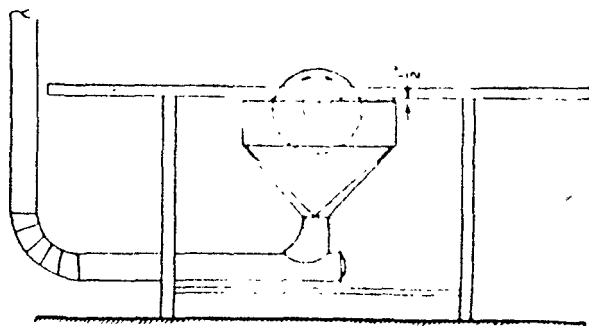
FIGURE 129. Local Exhaust at a Table Saw (Courtesy N. Y. Labor Department, Division Industrial Hygiene and Safety Standards)
