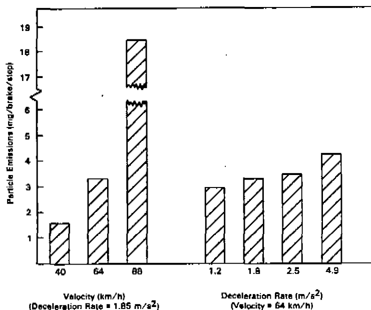
FIG. 4. Effect of velocity and deceleration rate on particle emissions from a disc brake.
