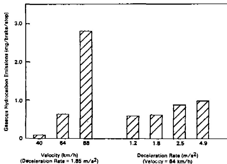
FIG. 5. Effect of velocity and deceleration rate on gaseous hydrocarbon emissions from a disc brake.
