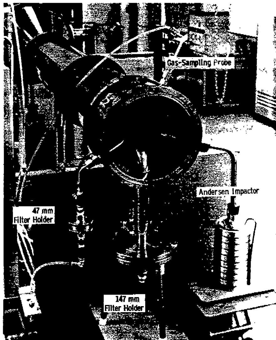
FIG. 3. Sampling probes for brake emission studies.
