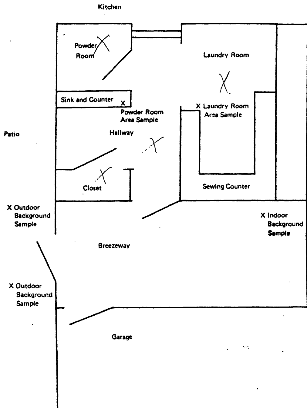
Figure 3 SITE PLAN - TEST SITE NO. 3
