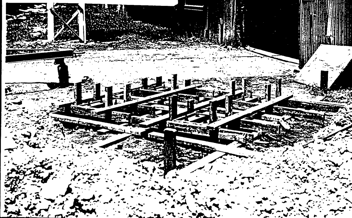
Dense Phase Booster Station Foundations Looking North, Auth #731241 5-2-74
