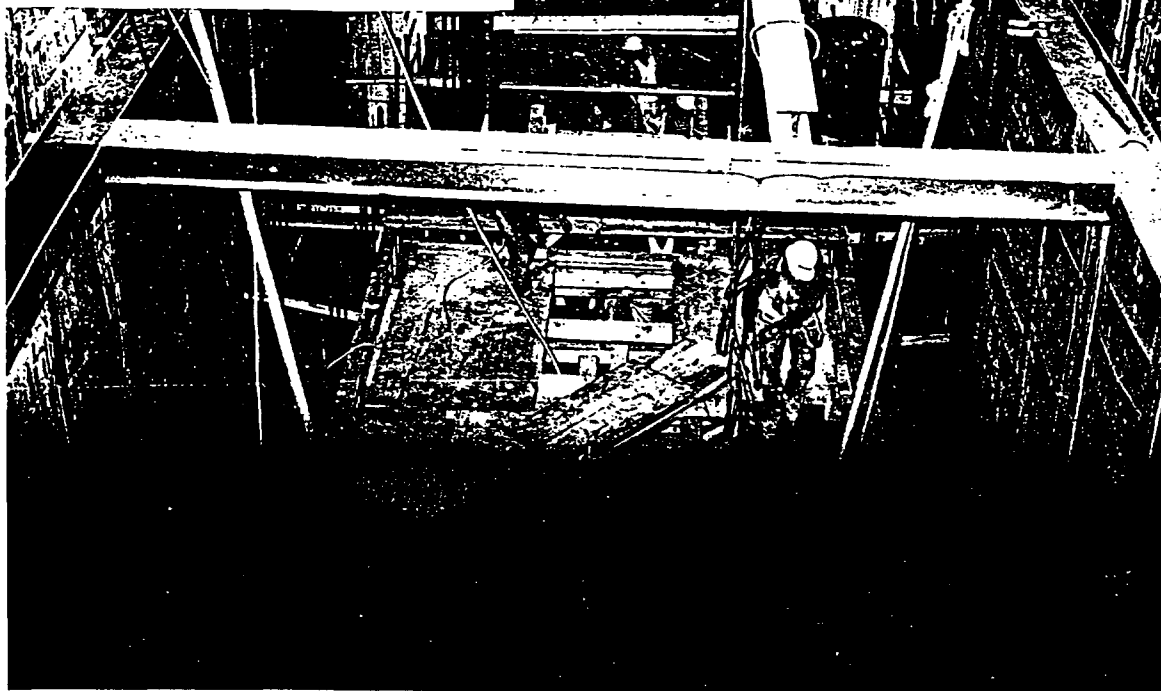
Casting Foundation, Casting Pit Looking North, Building 034 7-25-73
