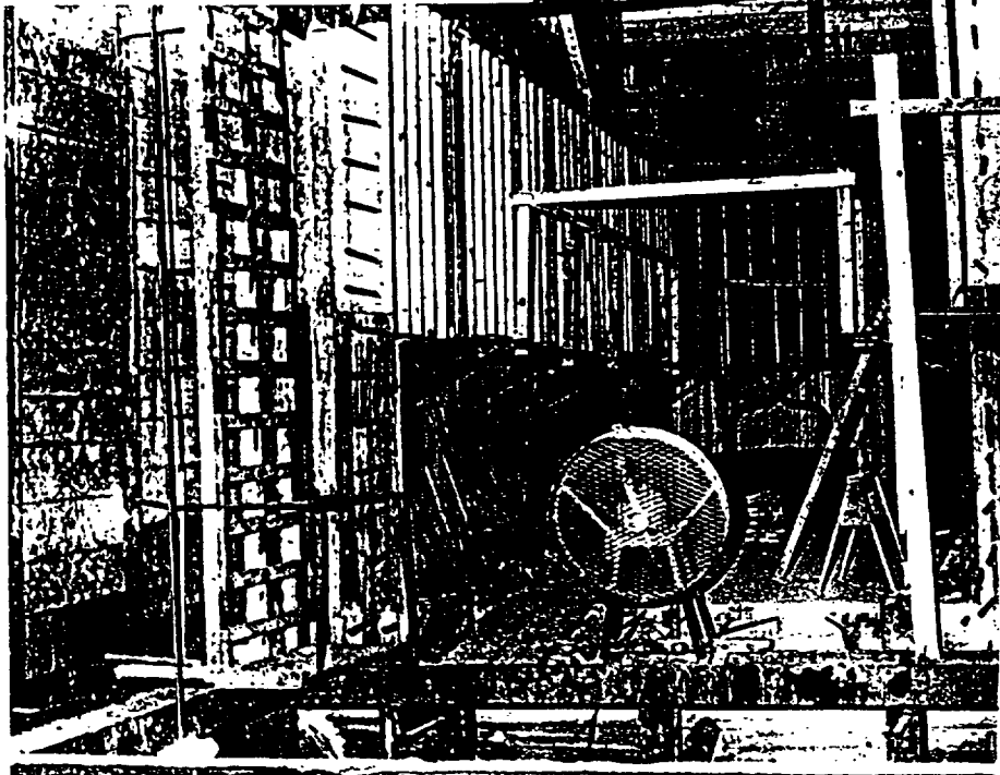
Casting Foundation Laydown Pit Looking North 6-20-73
