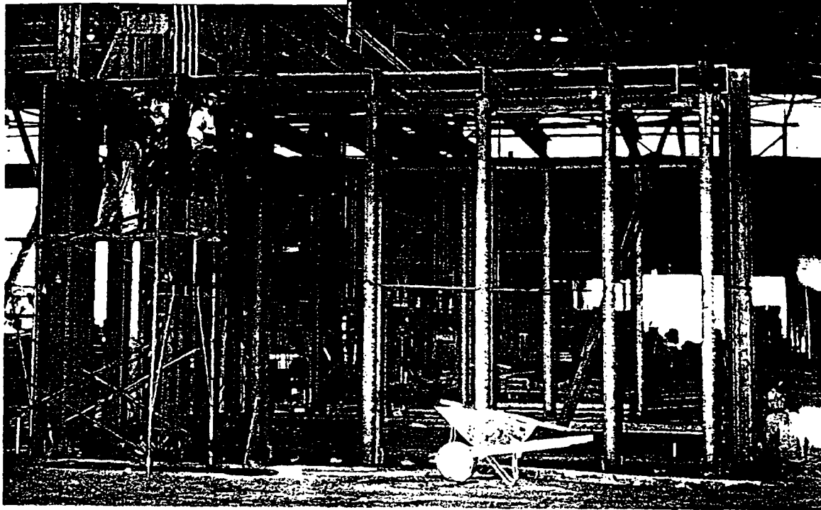
Furnace #9, Steel Erection Building 034-W 10-10-73
