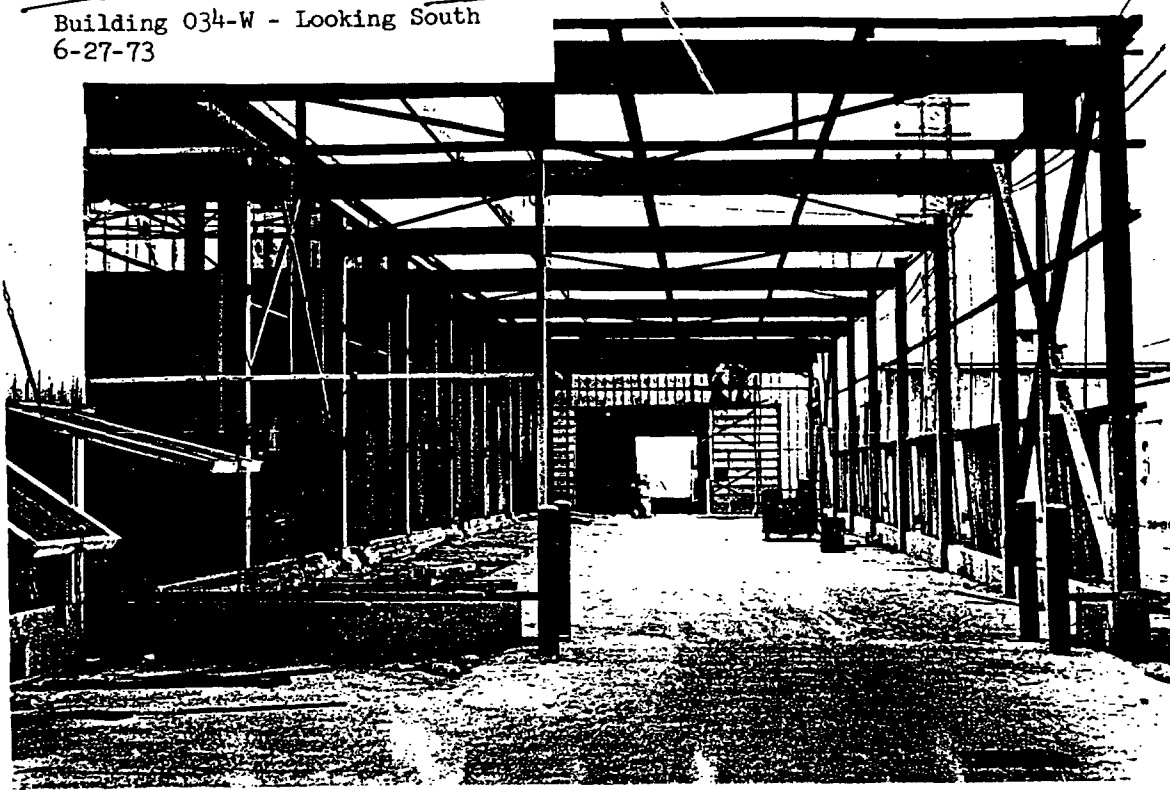
Casting Foundation - Casting Pit Building 034 6-27-73
