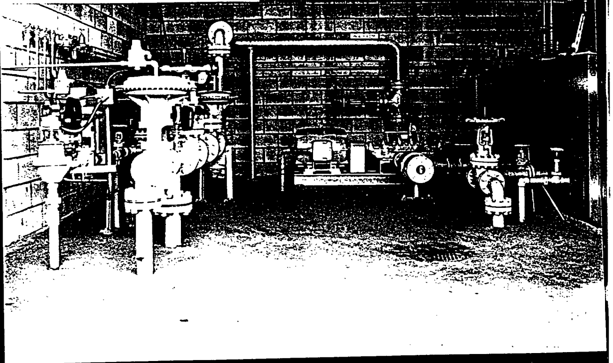
Building 34-H Hydraulic System Looking West, 2-20-74 Auth. #720769
