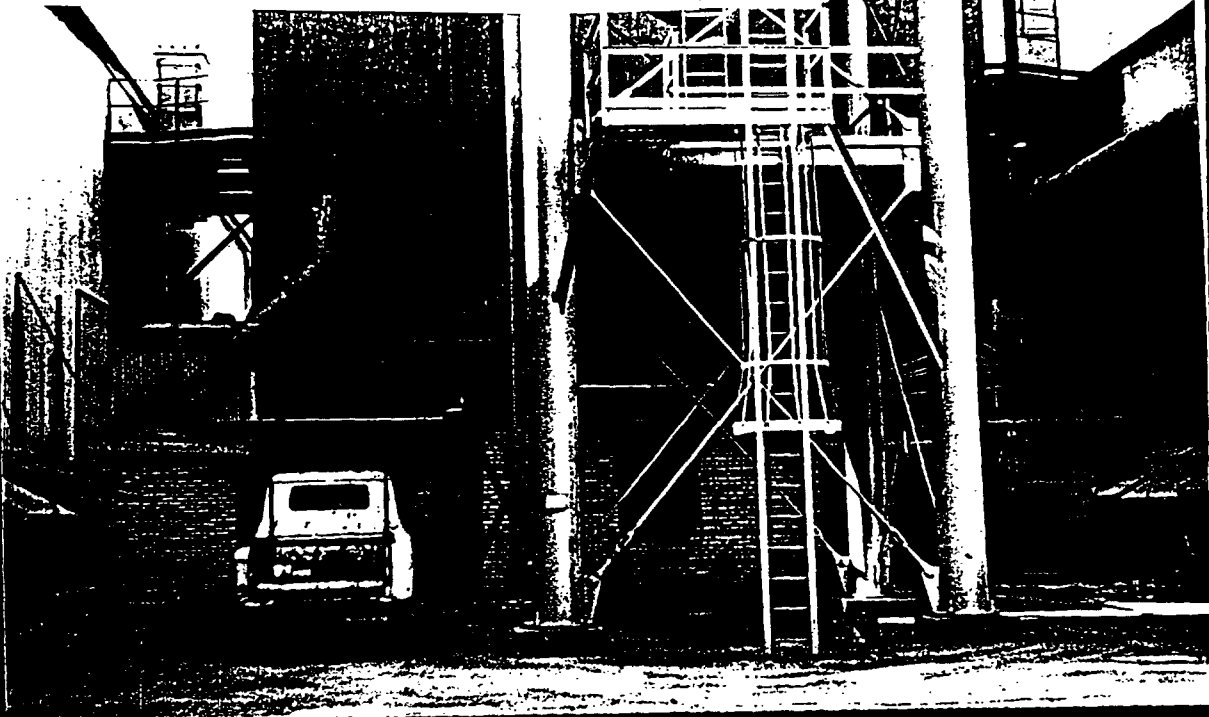
Reacted Ore Tank and Dust Collector Supports Building 21, 1-16-74 Auth. RS-730256
