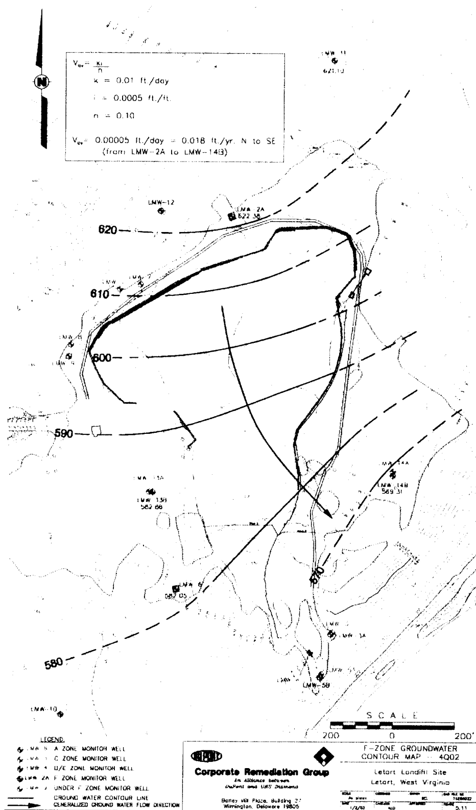
Figure 3.9: Letart Landfill Zone F Top-of-Groundwater Map.
