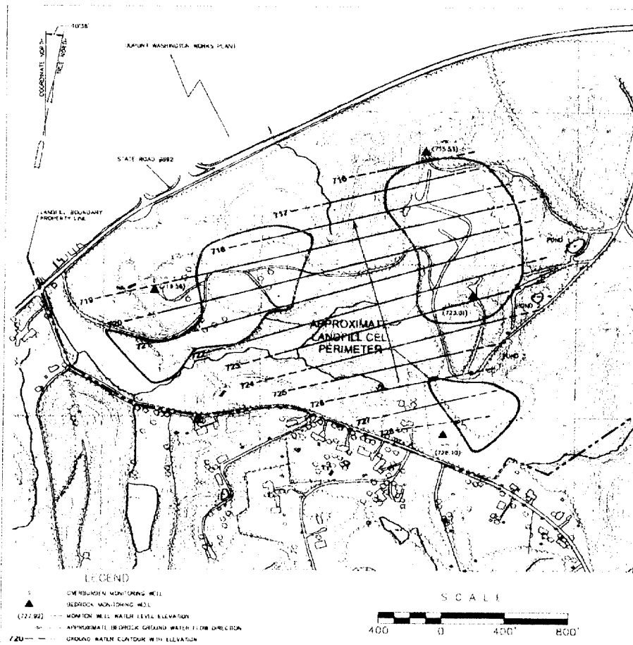
Figure 4.6: Local Landfill Zone A Top-of-Groundwater Map.
