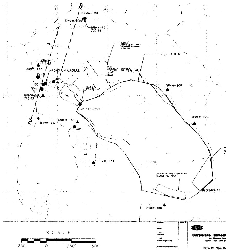
Figure 2.8: Dry Run Zone B Top-of-Groundwater Map.
