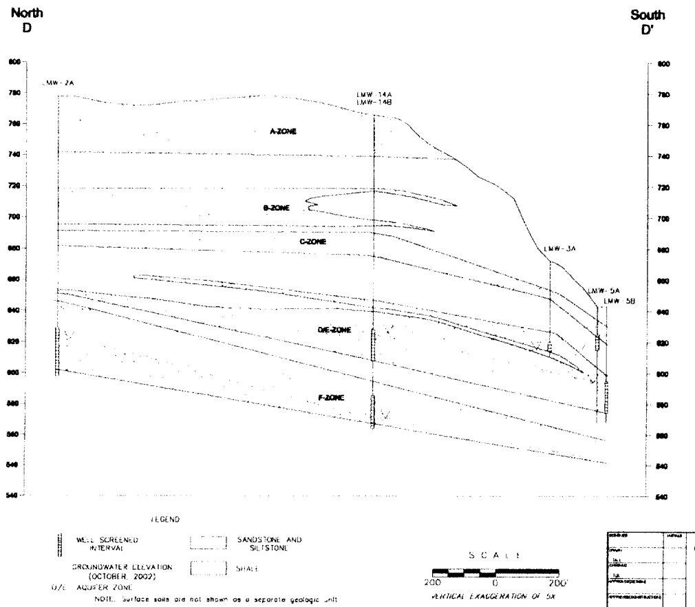
Figure 3.6: Letart Landfill Geological Cross-Section D-D'.
