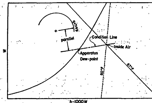
FIG. 9. ILLUSTRATION OF USE OF GOFF DIAGRAM IN SOLUTION OF EXAMPLE 12.
