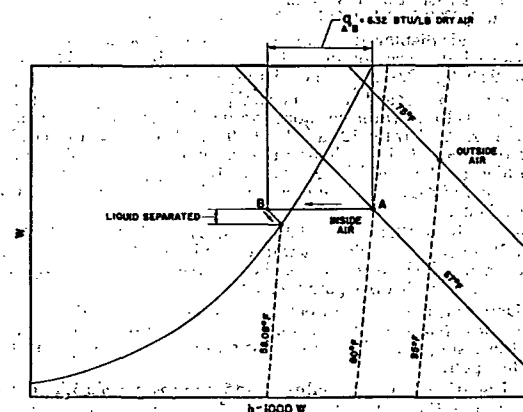
FIG. 10. ILLUSTRATION OF USE OF GOFF DIAGRAM IN SOLUTION OF EXAMPLE 13.
