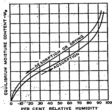
FIG. 5. TYPICAL EQUILIBRIUM MOISTURE CONTENT CURVES 1
