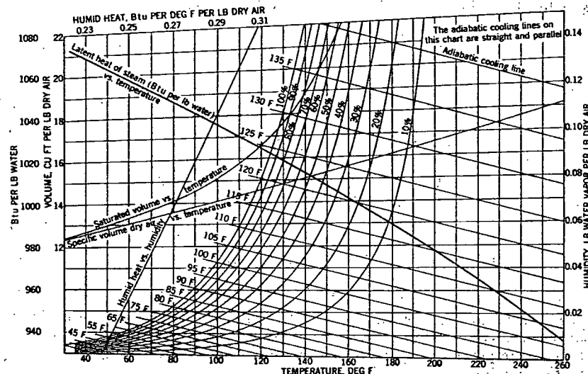
FIG. 6. PSYCHROMETRIC CHART
