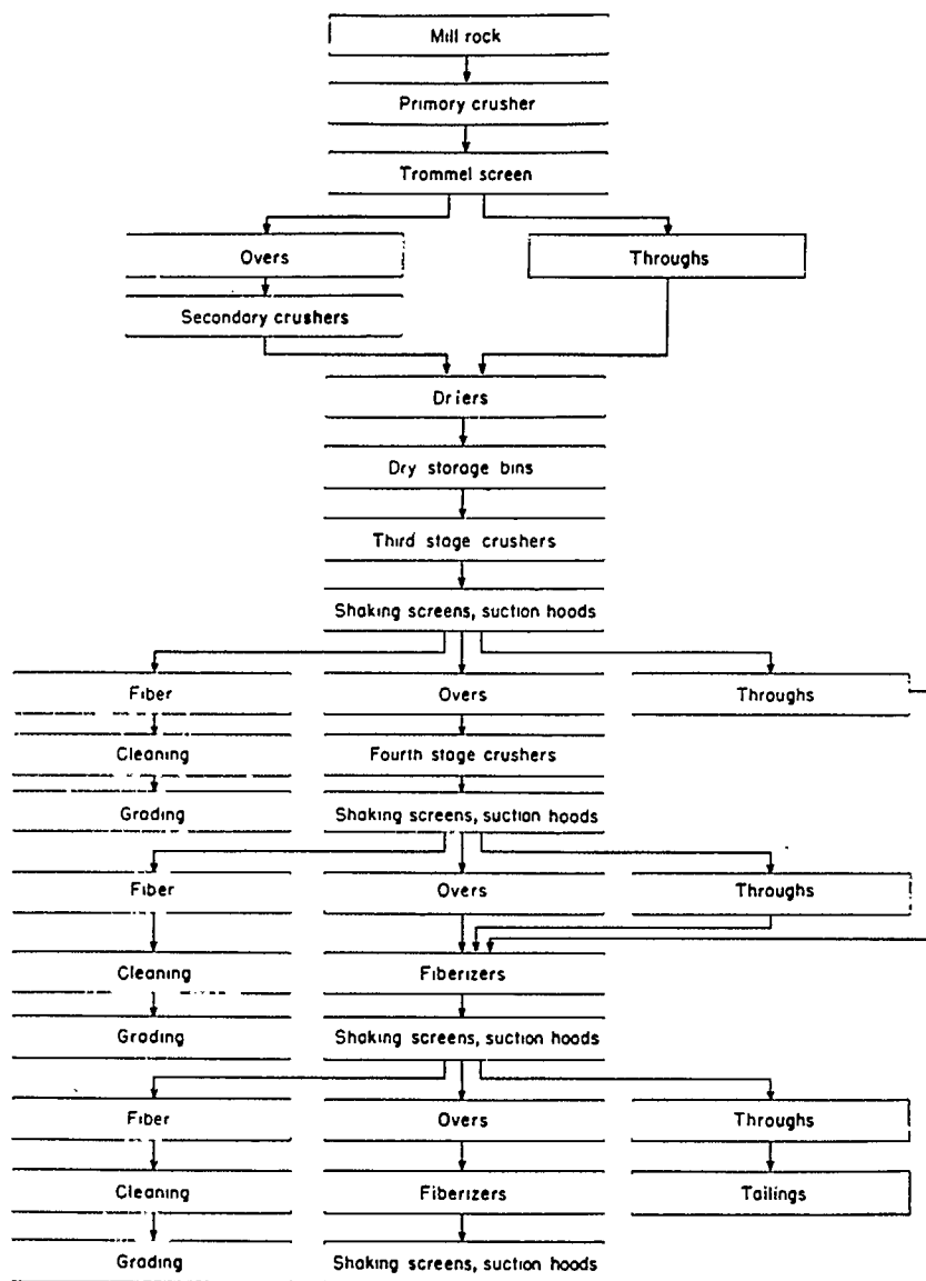
FIGURE 12.—Typical Flowsheet of a Canadian Asbestos Mill.
