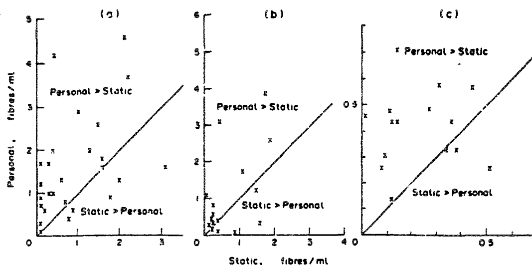
FIGS 3(a), (b) and (c). Personal vs static sampling results from Factory A. (a) First set of data. Samples not obtained simultaneously. (b) Second set. Each point represents mean of five 20 min static samples covering 3 hr personal sample on operative nearest (1–3 m) to static site. (c) Third set. Simultaneous static samples and operatives' personal samples at various machines. Each personal and static result is the mean from two samples (4 in one case).
