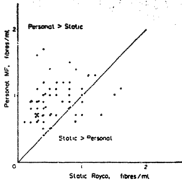
FIG. 4. Personal vs static sampling results from textile processes at Factory B. (Personal, 4 hr MF samples Static, 15 min Royco counts taken on same day as personal samples.
