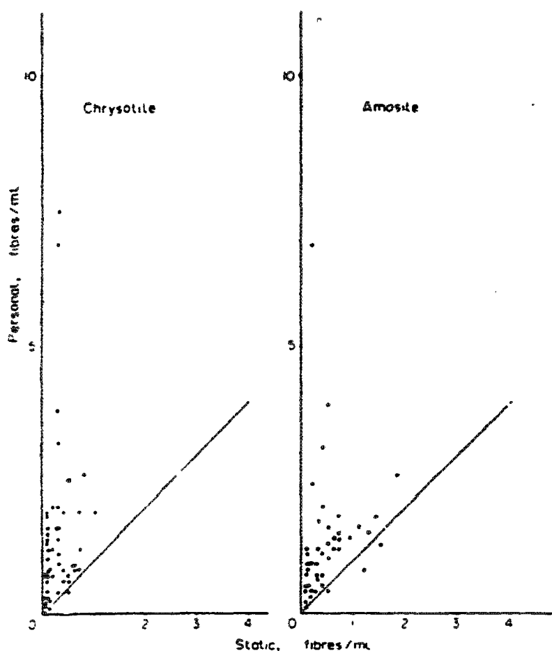
FIG 6 Personal vs static sampling results from Factory D classified by asbestos type. Various operations; mostly overlapping sampling periods; distances between instruments mostly in range 6–15 m.
