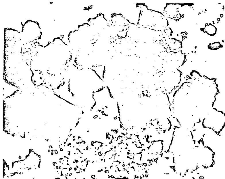
Fig. 6. Specimen I37. Carbonate in talc inclusion x 3000. Compact particles together with some plate-like forms and rolled talc sheets.
