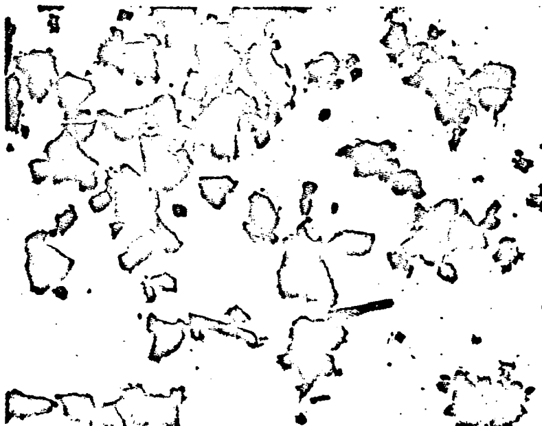
Fig. 4. Specimen I21. Inclusion from Face 2. x 3000. This specimen produced plate-like and compact particles with some lath-like forms.
