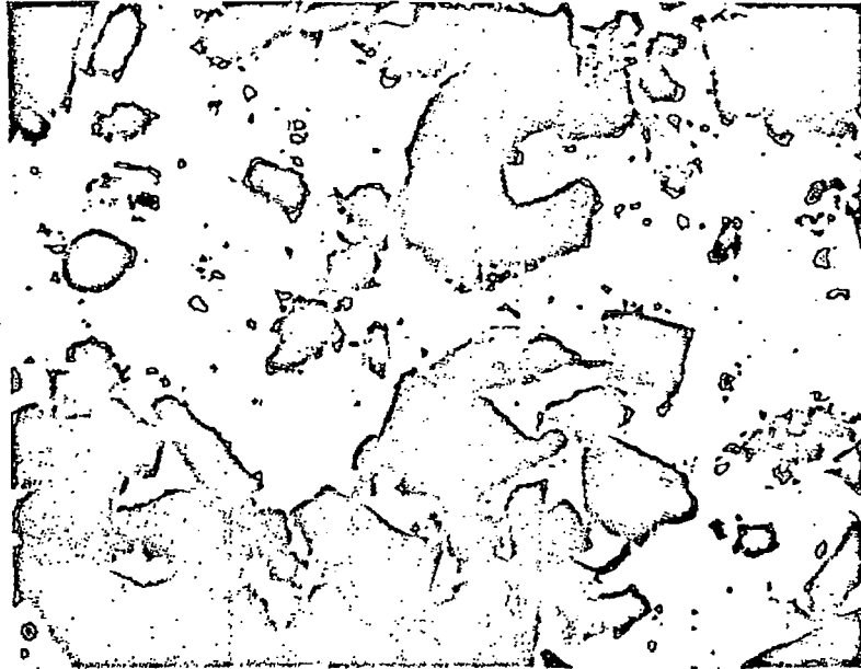
Fig. 9. Specimen I32. Face 2 inclusion from base of talc seam, x 3000. The specimen produced a mixture of irregular particles varying from compact to plate-like in form with a few lath like particles.
