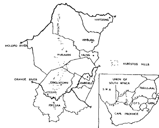
FIG. 1. Map of Grouped West asbestos fields.
