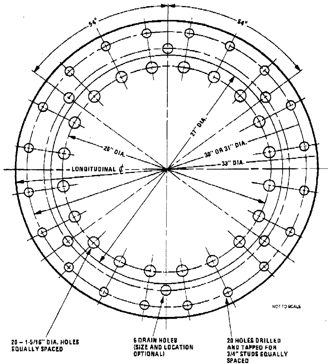
FIGURE 2.2 STANDARD MANWAY COVER FOR 20" MANWAY VCM TANK CARS
