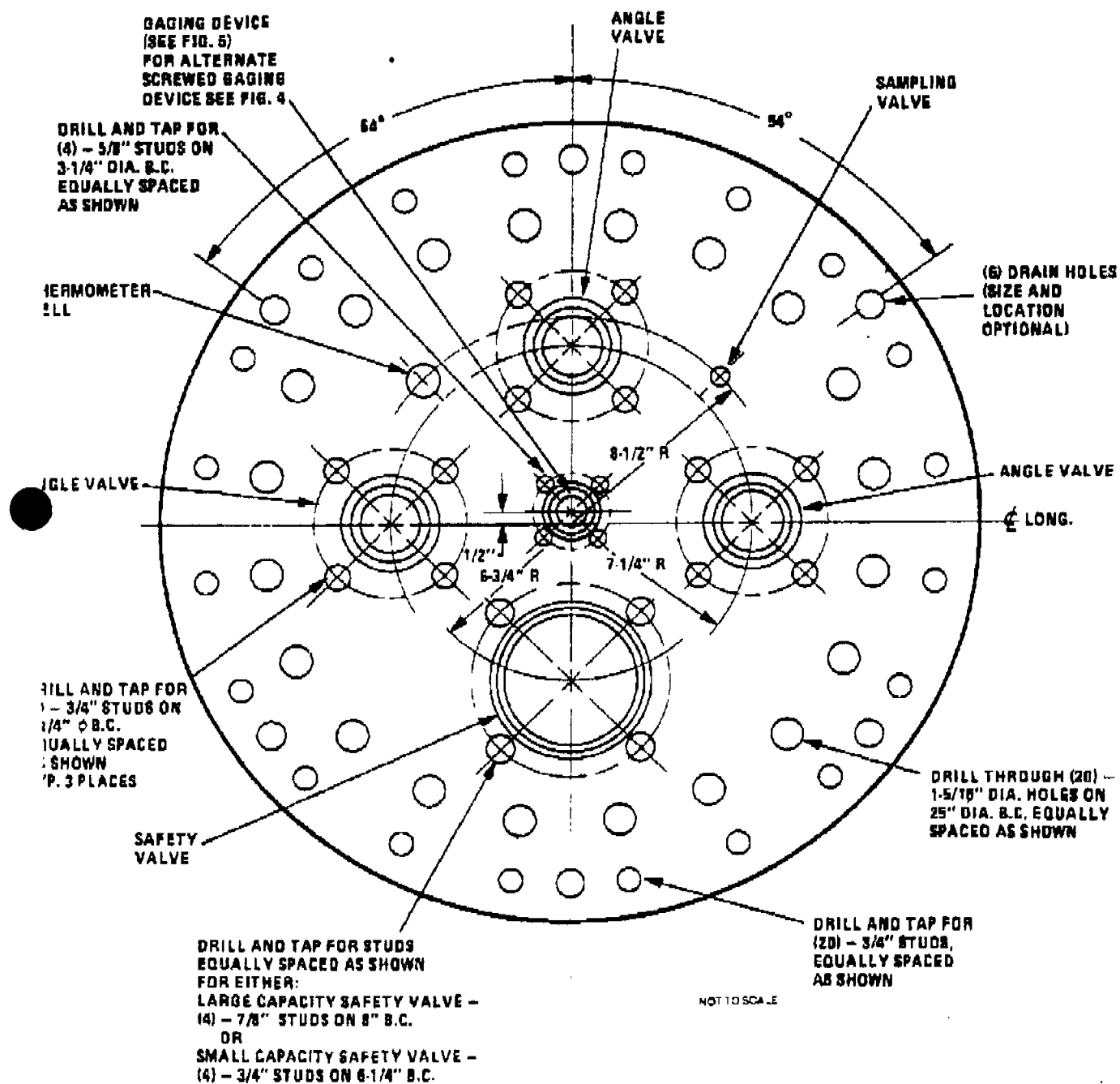
FIGURE 2.1 STANDARD MANWAY COVER FOR 20" MANWAY VCM TANK CARS
