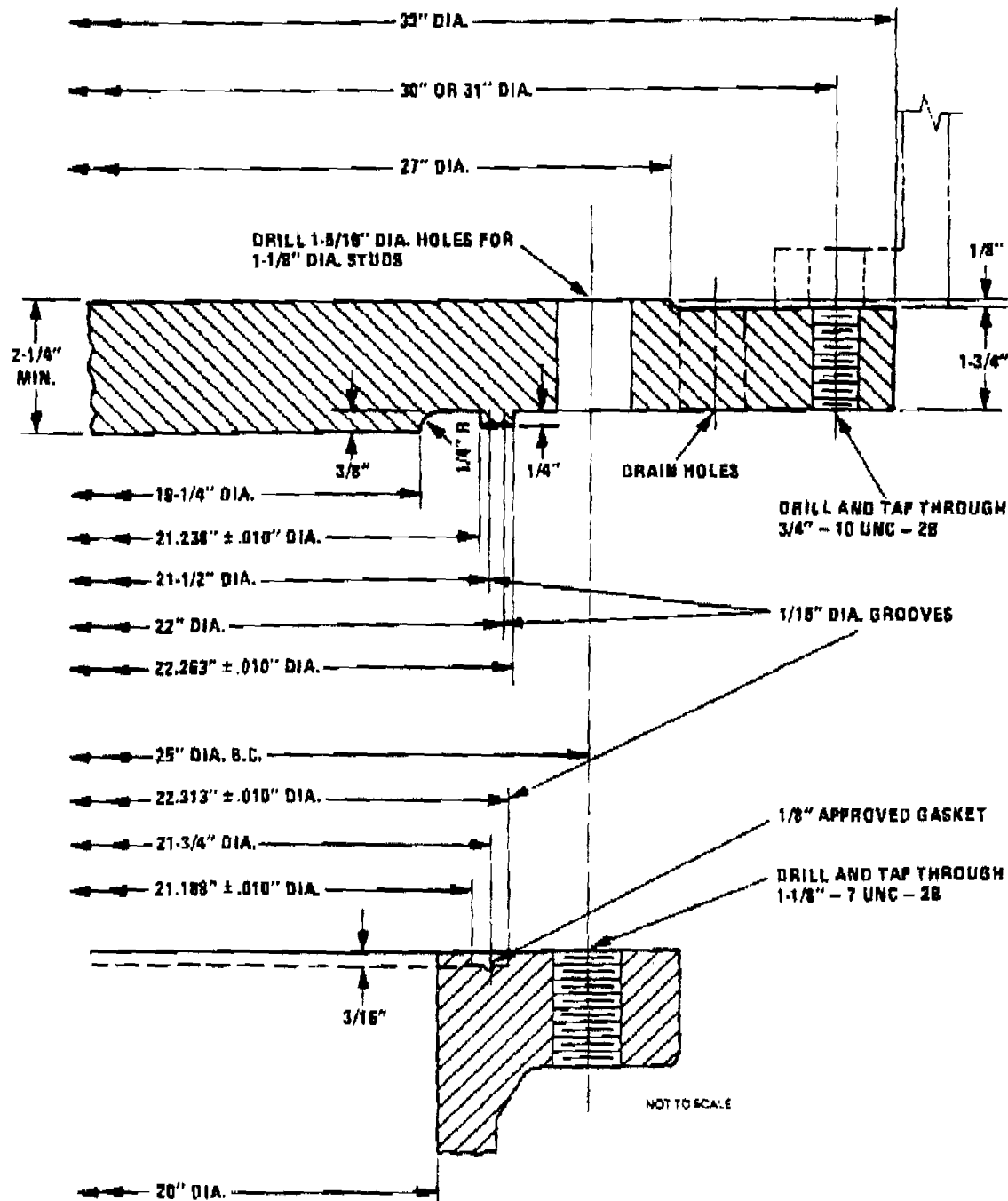
FIGURE 2.3 DETAIL OF COVER AND NOZZLE JOINT FOR 20" MANWAY VCM TANK CARS
