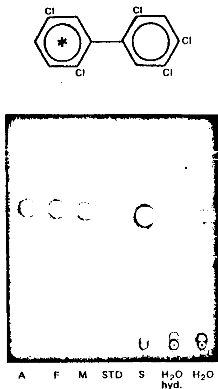
Fig. 2C. Radioautogram of TLC plate containing extracts of water and organisms treated with 2,4,5,2',5'-pentachlorobiphenyl. A (alga), F (fish), M (mosquito larva), S (snail) and STD ( 14 C-radiolabeled compound).
