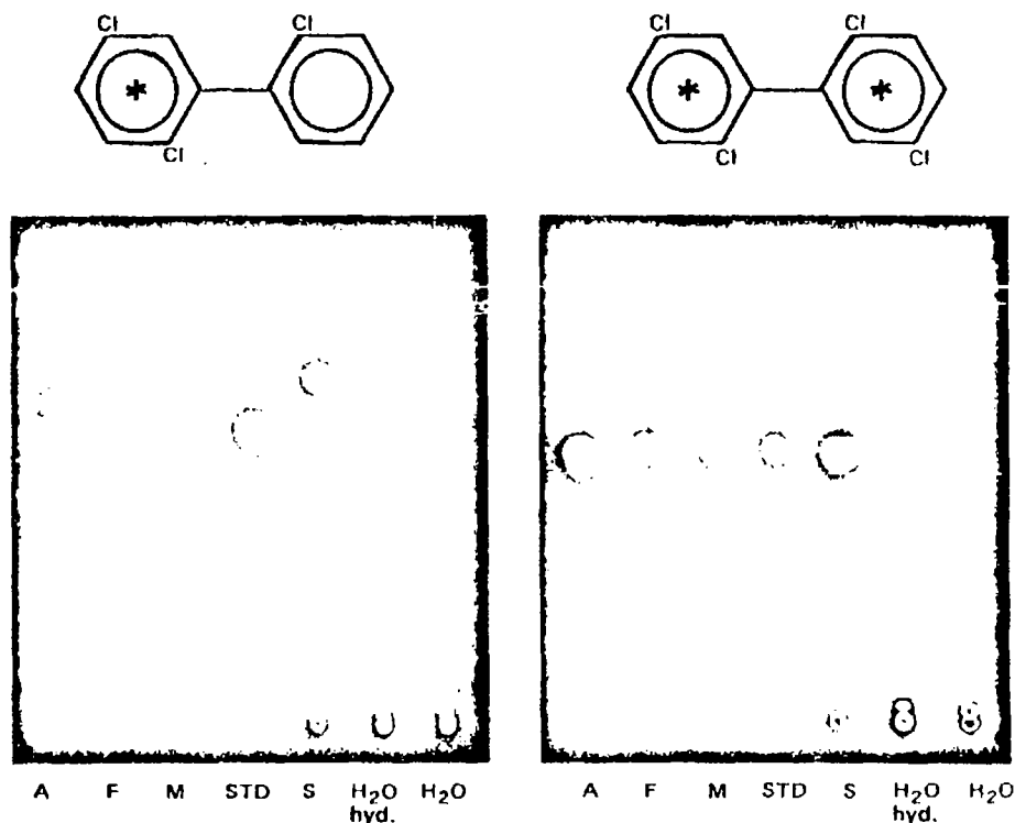
Fig. 2A. Radioautogram of TLC plate containing extracts of water and organisms treated with 2,5,2'-trichlorobiphenyl. A (alga), F (fish), M (mosquito larva), S (snail) and STD ( ^{14}\text{C} -radiolabeled compound).
