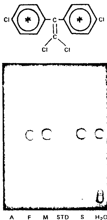
Fig. 2D. Radioautogram of TLC plate containing extracts of water and organisms treated with DDE. A (alga), F (fish), M (mosquito larva), S (snail) and STD ( 14 C-radiolabeled compound).
