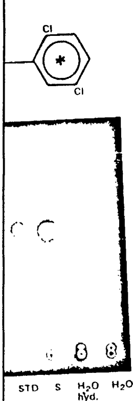
Radioautogram of TLC plate containing extracts of water and organisms treated with 2,4,5,2',5'-tetrachlorobiphenyl. A (alga), F (fish), M (mosquito larva), S (snail) and STD ( 14 C-radiolabeled compound).
