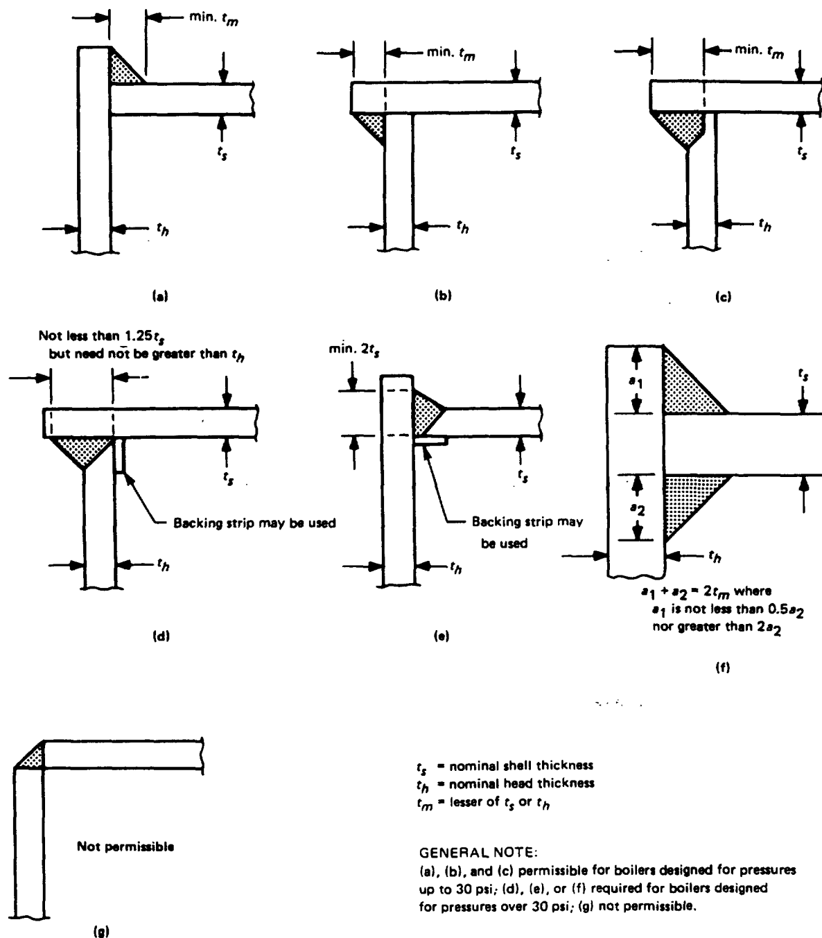
FIG. HW-701.3 SOME FORMS OF ATTACHMENTS OF PRESSURE PARTS TO FLAT PLATES TO FORM A CORNER JOINT (TEE JOINT)
