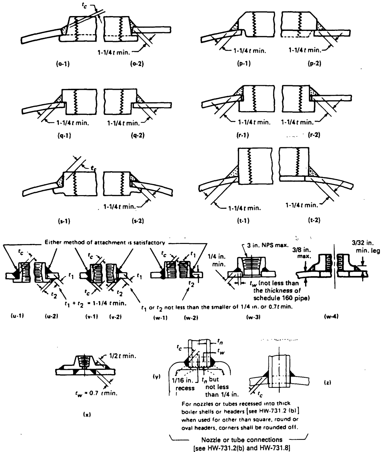
FIG. HW-731 SOME ACCEPTABLE TYPES OF WELDED NOZZLES AND OTHER CONNECTIONS TO SHELLS, DRUMS, AND HEADERS (CONT'D)
