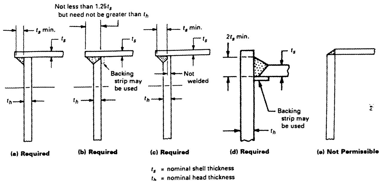
FIG. HLW-401.2 TYPICAL CORNER JOINTS
