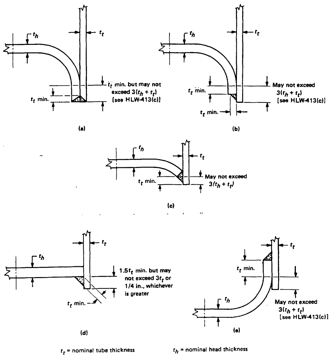
FIG. HLW-413 TUBES ATTACHED BY WELDING
