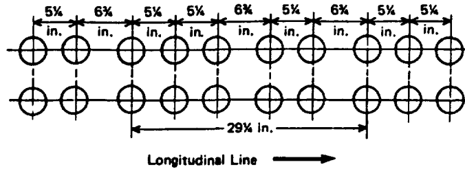
FIG. HG-350.3 EXAMPLE OF TUBE SPACING WITH PITCH OF HOLES VARYING IN EVERY SECOND AND THIRD ROW
