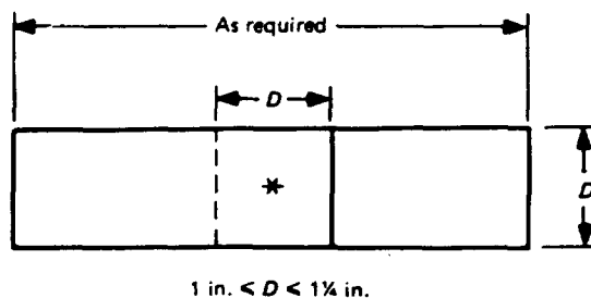
(b) Single-Spot-Weld Tension Specimen, Two-Ply Joint
