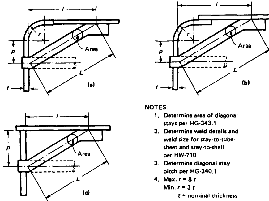
FIG. HG-343 DETAILS OF INSTALLATION OF DIAGONAL STAYS
