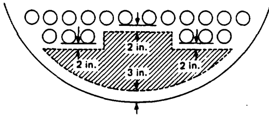
FIG. HG-345.2 METHOD OF DETERMINING NET AREA OF IRREGULAR SEGMENT OF A HEAD
