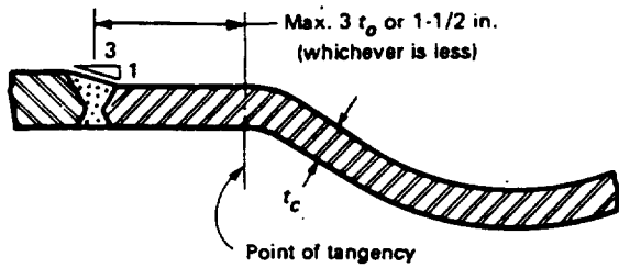
FIG. HG-312.6 CONNECTION BETWEEN PLAIN AND CORRUGATED FURNACE
