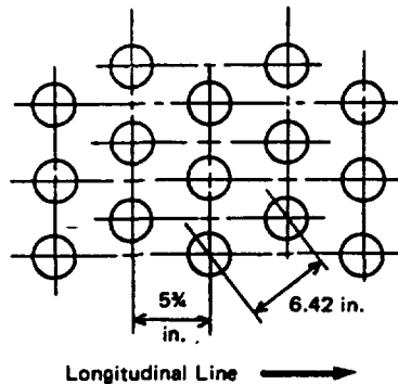
FIG. HG-350.4 EXAMPLE OF TUBE SPACING WITH TUBE HOLES ON DIAGONAL LINES
