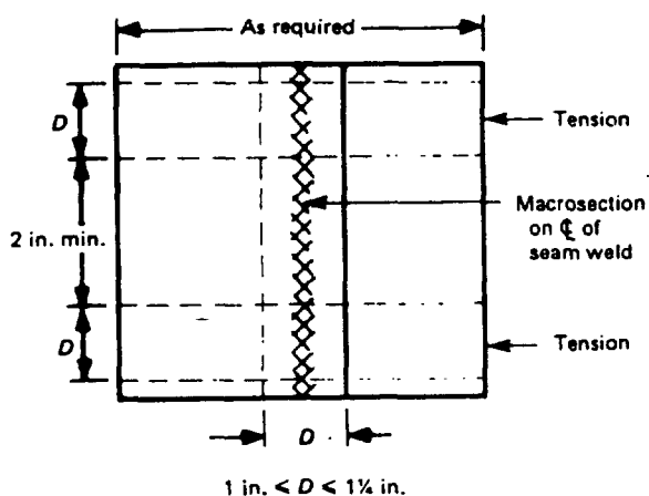
(c) Seam-Weld Specimen for Tension and Macrosection, Two-Ply Joint
