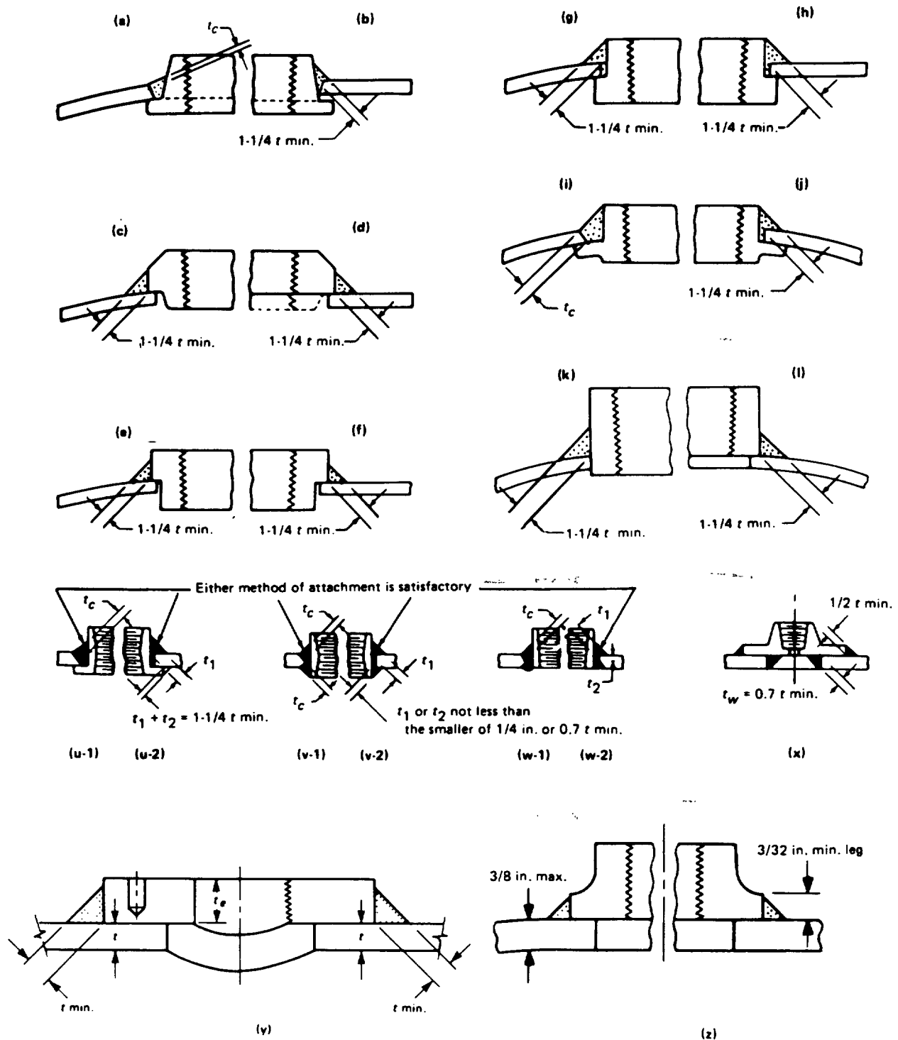
FIG. HLW-431.5 SOME ACCEPTABLE TYPES OF WELDED NOZZLES AND OTHER CONNECTIONS TO SHELLS AND HEAD
