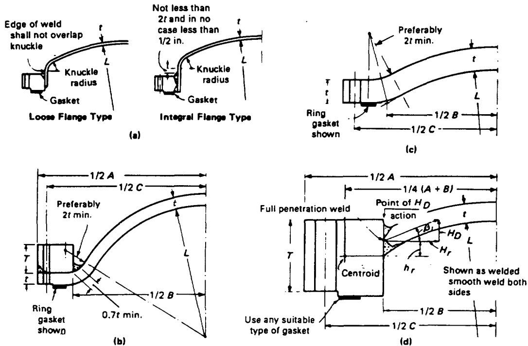
FIG. HG-309 SPHERICALLY DISHED STEEL PLATE COVERS WITH BOLTING FLANGES
