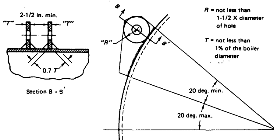
FIG. HG-725(b) WELDED BRACKET CONNECTION FOR HORIZONTAL-RETURN TUBULAR BOILER
