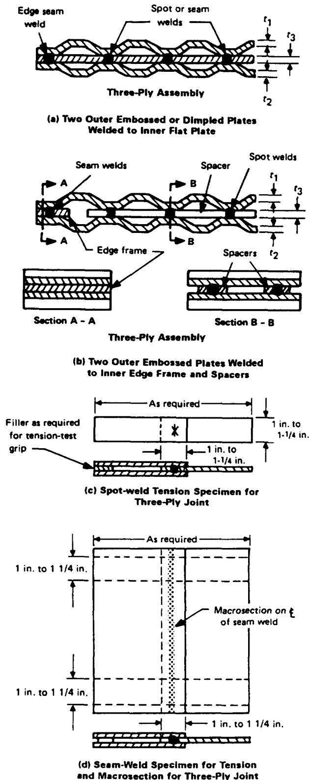
FIG. HW-740 THREE-PLY JOINT ASSEMBLIES
