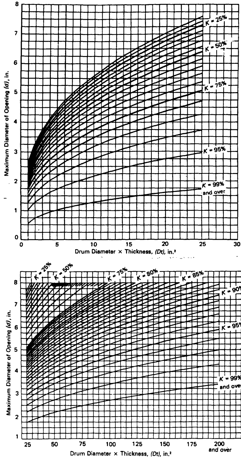
FIG. HG-320 CHART SHOWING LIMITS OF SIZES OF OPENINGS WITH INHERENT COMPENSATION IN CYLINDRICAL SHELLS Maximum Permissible Diameter of Opening Is 8 in.
