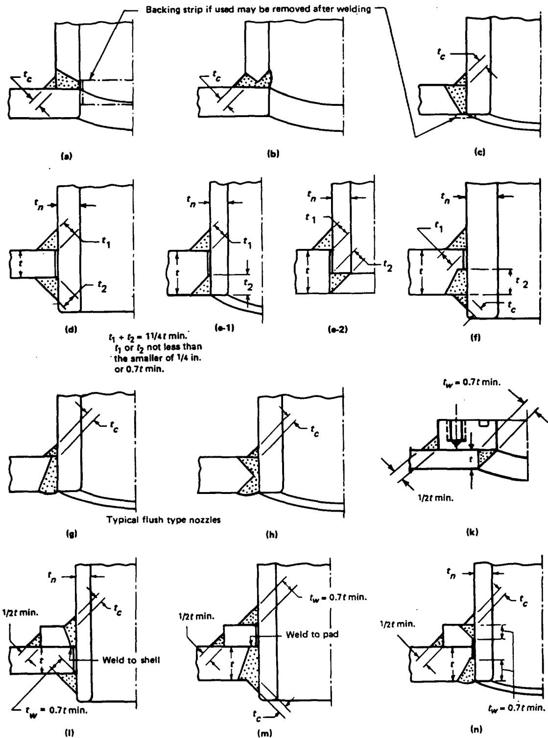
FIG. HW-731 SOME ACCEPTABLE TYPES OF WELDED NOZZLES AND OTHER CONNECTIONS TO SHELLS, DRUMS, AND HEADERS
