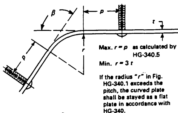
FIG. HG-340.1 PITCH OF STAYBOLTS ADJACENT TO UPPER CORNERS OF FIREBOXES
