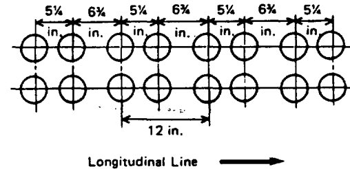
FIG. HG-350.2 EXAMPLE OF TUBE SPACING WITH PITCH OF HOLES UNEQUAL IN EVERY SECOND ROW
