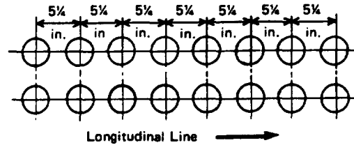
FIG. HG-350.1 EXAMPLE OF TUBE SPACING WITH PITCH OF HOLES EQUAL IN EVERY ROW
