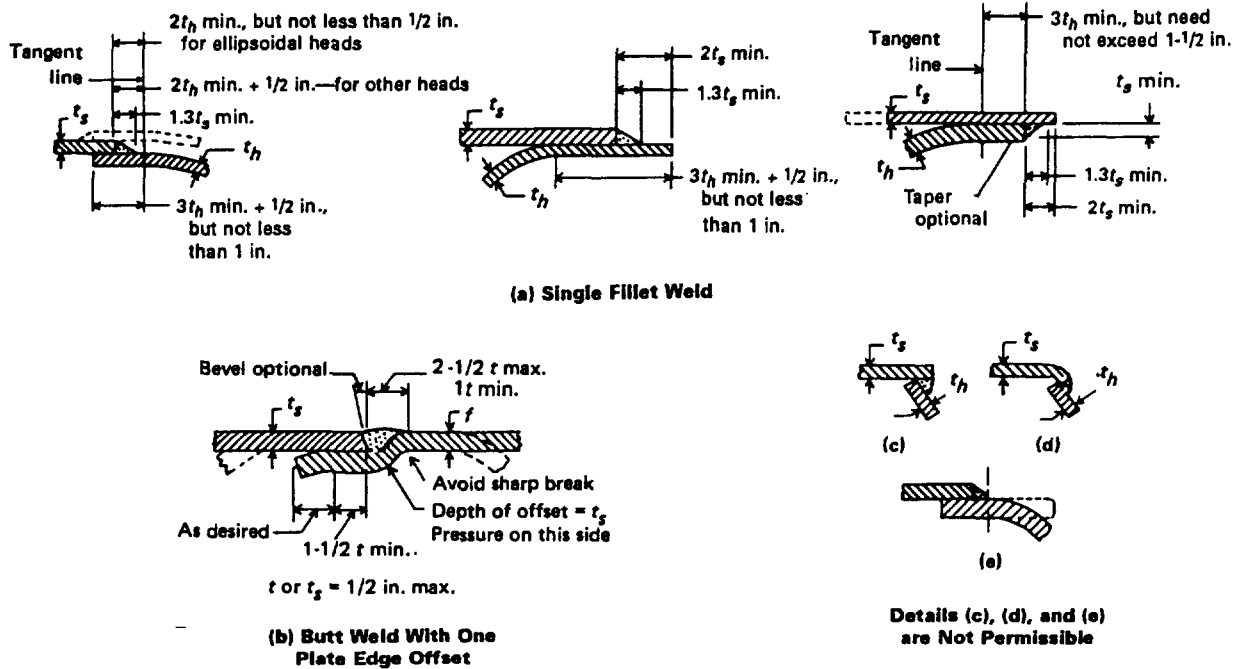
FIG. HW-715.1 HEADS ATTACHED TO SHELLS
