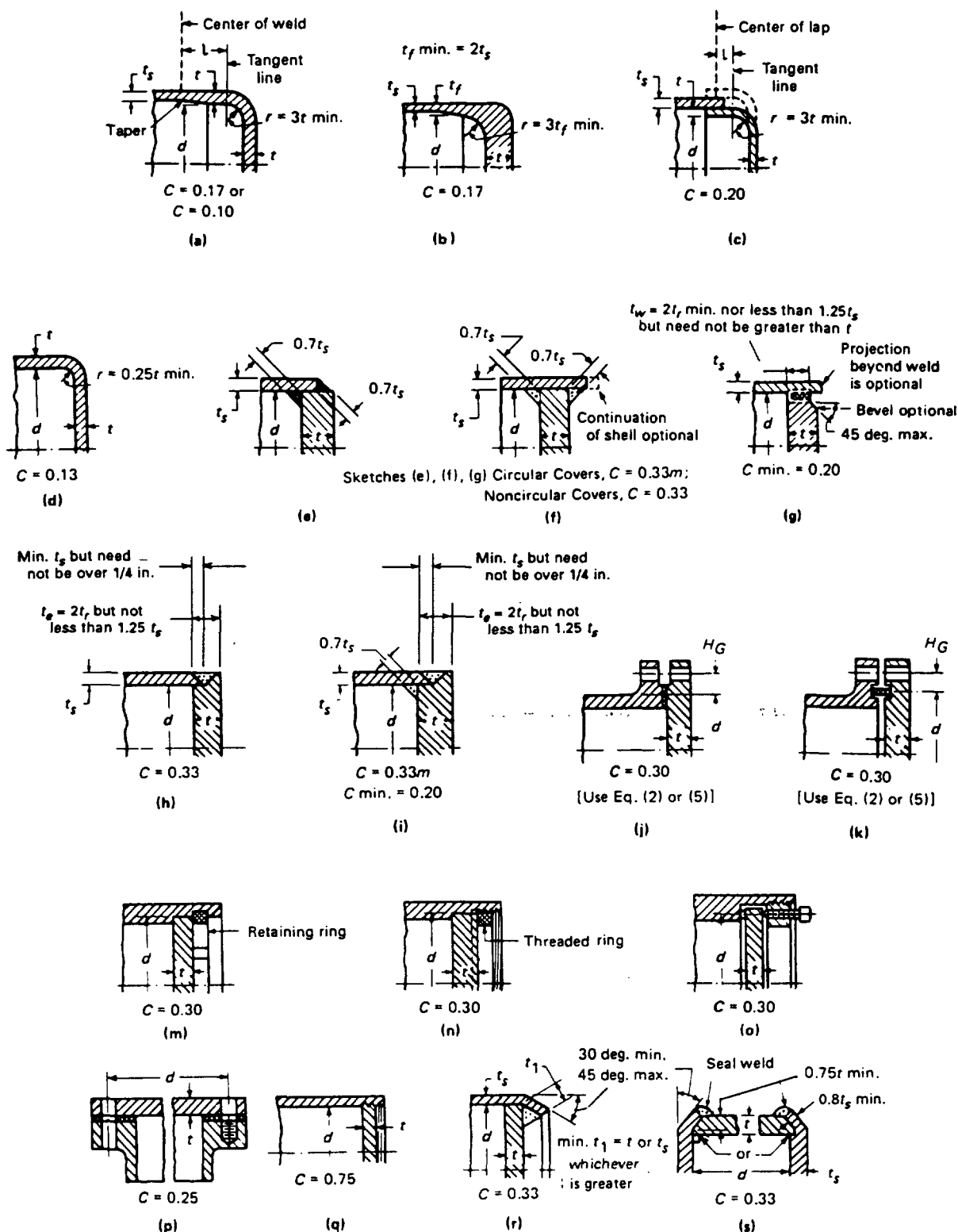
FIG. HG-307 SOME ACCEPTABLE TYPES OF UNSTAYED FLAT HEADS AND COVERS The Above Illustrations Are Diagrammatic Only. Other Designs Which Meet the Requirements of HG-307 Will Be Acceptable.
