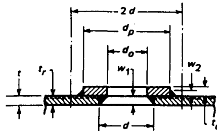
FIG. D-100 COMPUTATION OF TYPICAL PAD REINFORCEMENT
