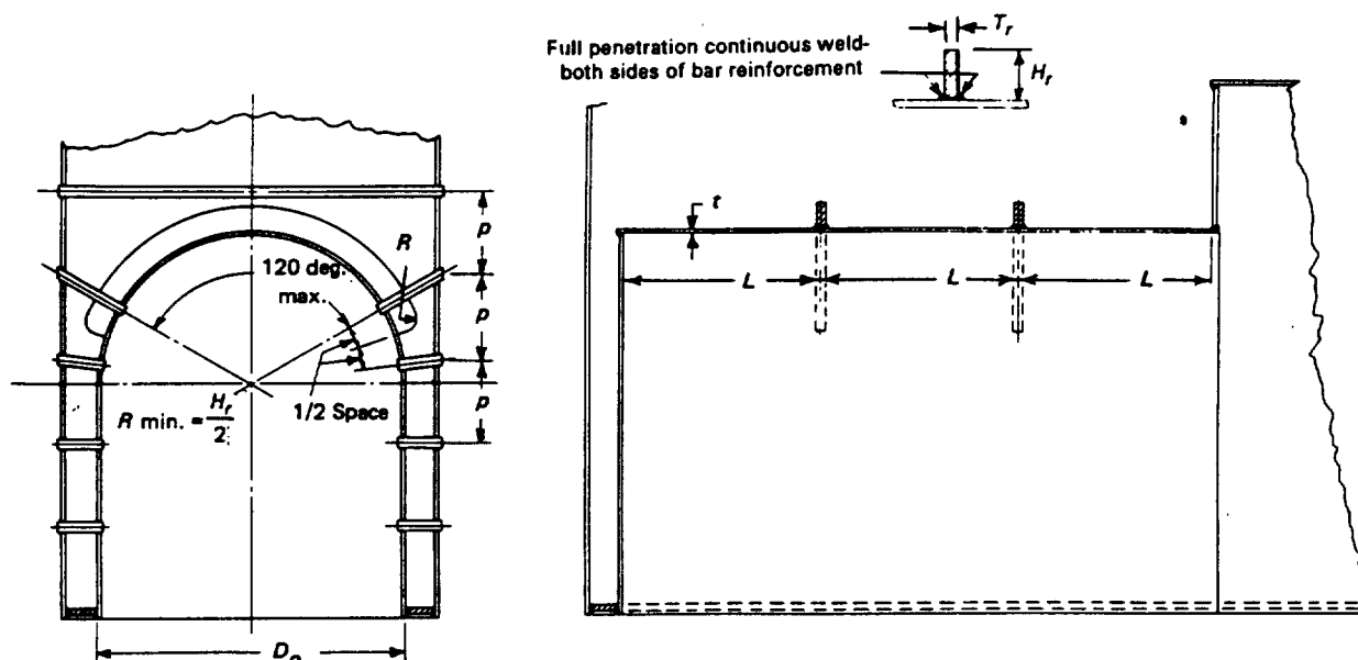
FIG.-HG-312.7 ACCEPTABLE TYPE OF SEMICIRCULAR FURNACE REINFORCEMENT
