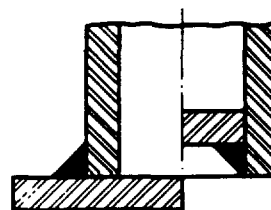
FIG. HG-340.3 EXAMPLES OF ACCEPTABLE CORNER WELDS FOR PRESSURES NOT OVER 30 psi
