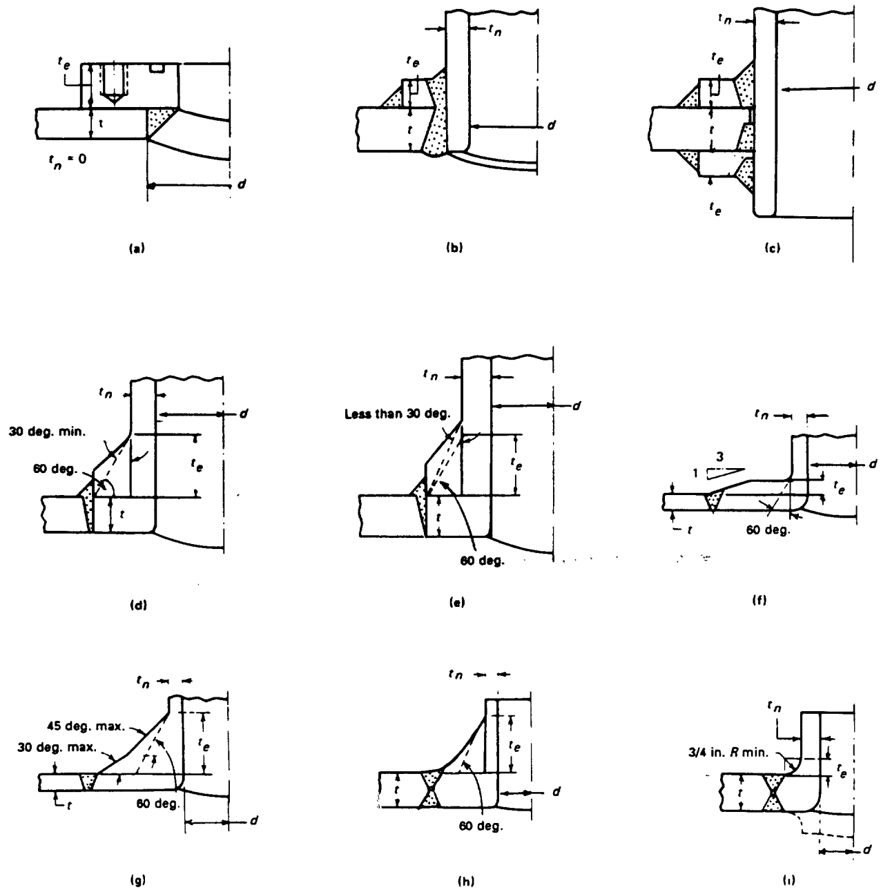
FIG. HG-326 SOME REPRESENTATIVE CONFIGURATIONS DESCRIBING THE \ell_r REINFORCEMENT DIMENSION
