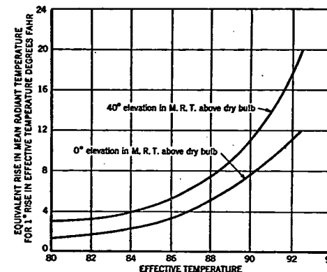
FIG. 4. EFFECT OF MRT ELEVATION IN TERMS OF EFFECTIVE TEMPERATURE
