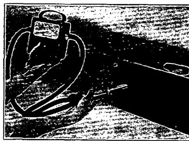
Fig. 2—Showing Tube Type Velometer with Duct Jet taking readings directly in the duct. Duct Jet furnished 18 in. or 36 in. long
