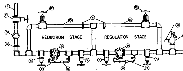
PLAN VIEW
