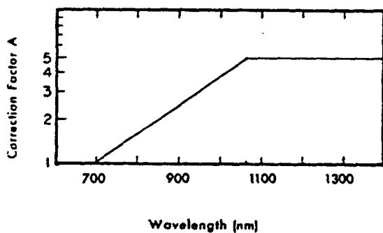
Figure 2 — TLV correction factors for laser wavelengths (eye).
