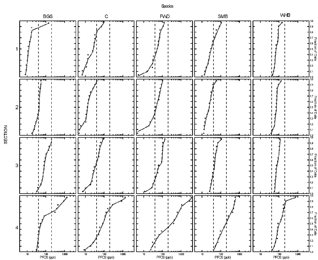
Figure 6 PFOS in Species-Section Matrix; vertical bars are 40 ppt and 200 ppt
