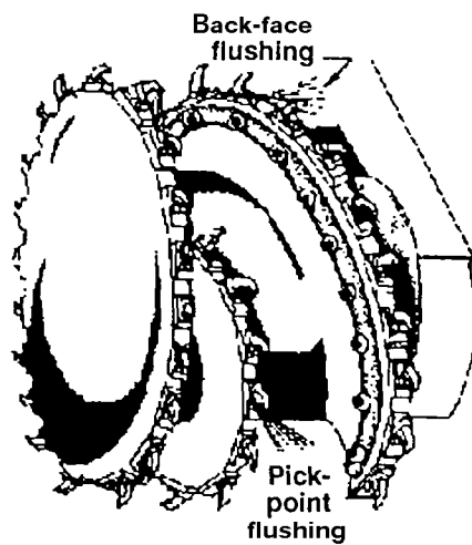
Figure 7. Pick-point flushing
