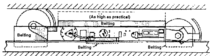
Figure 6. Air-splitting screens
