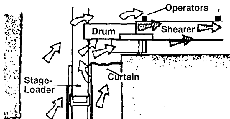
Figure 5. Cut-out curtain
