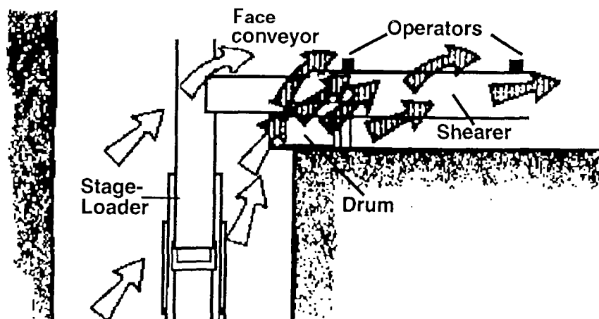
Figure 4. Dust rollback
