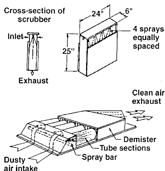
Figure 13. Spot scrubbers
