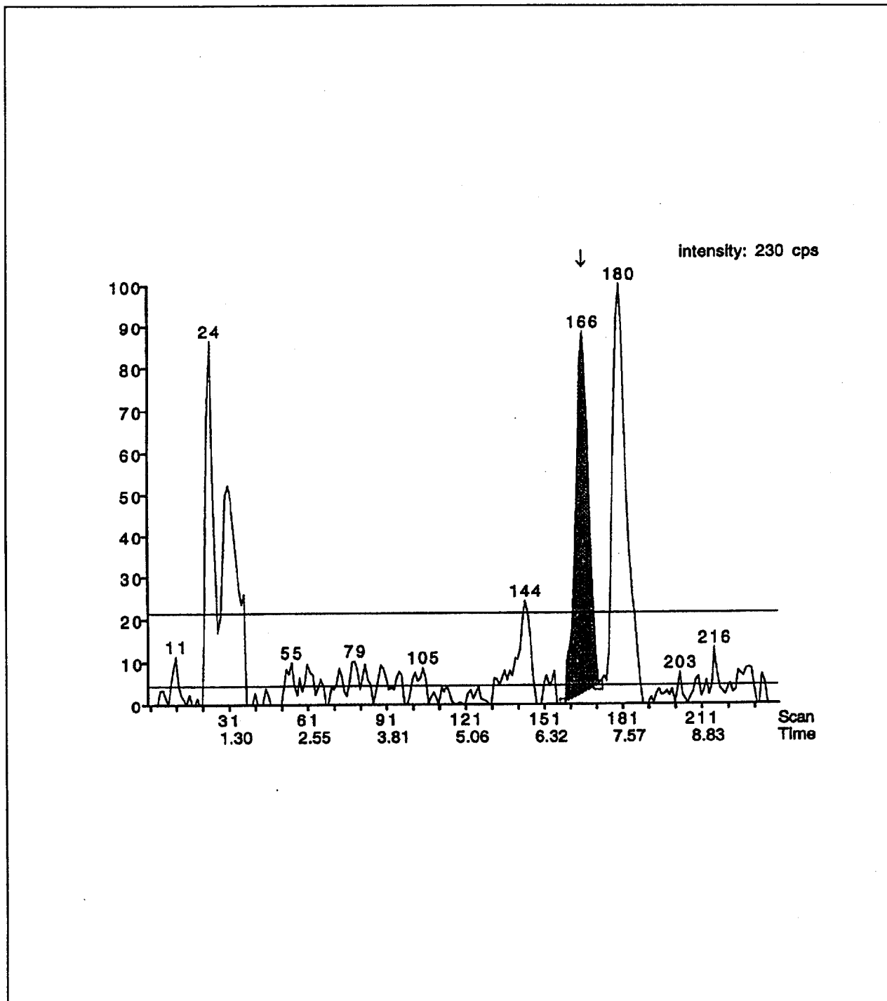
Figure 5. A representative chromatogram of a matrix blank sample (454-102-MAB-1). The arrow indicates the retention time of PFOS.
